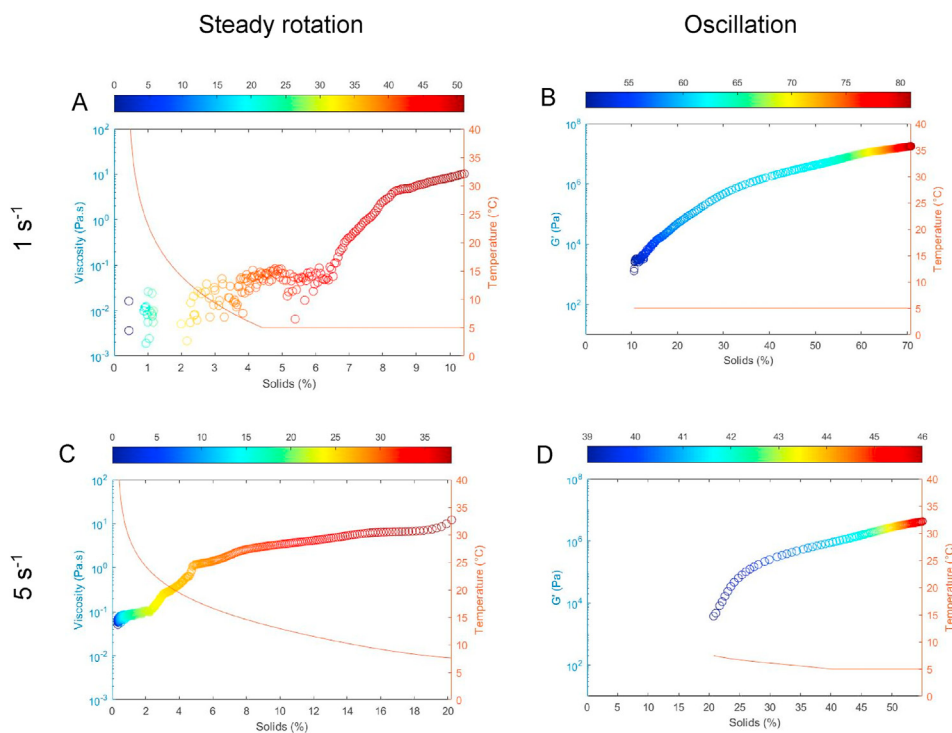
Fig. 6. Apparent viscosity at a shear rate of 1 \text{ s}^{-1} (A) and 5 \text{ s}^{-1} (C) and storage modulus at an oscillatory deformation of 0.005% (B, D) as a function of the amount of solids in sPMF. The color in the apparent viscosity curves ranges from dark blue at 0 min to dark red at 51 (A) or 38 min (C), whereas the color in the G' -curves starts at dark blue at the end of the rotation experiment and extends to dark red at 81 min (B) or 46 min (D). (For interpretation of the references to color in this figure legend, the reader is referred to the Web version of this article.)
