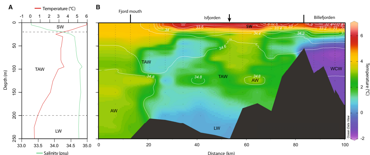
Fig. 2. Conductivity, temperature, depth (CTD) profiles of Isfjorden. AW = Atlantic Water; TAW = Transformed Atlantic Water; WCW = Winter Cooled Water; LW = Local Water; SW = Surface Water. A. CTD profile taken in July 2018 at the station 19272345 (B) ( 78^{\circ}18.3'N ; 15^{\circ}25.38'E ), close to core HH16-1205-GC site. B. CTD section from Isfjorden mouth to Billefjorden along the southern side of the fjord in July 2018. Salinity is given by white contour lines. The black arrow points to the location of station 19272345 (B). Data were retrieved from World Ocean Database 2018 (Boyer et al. 2018).
