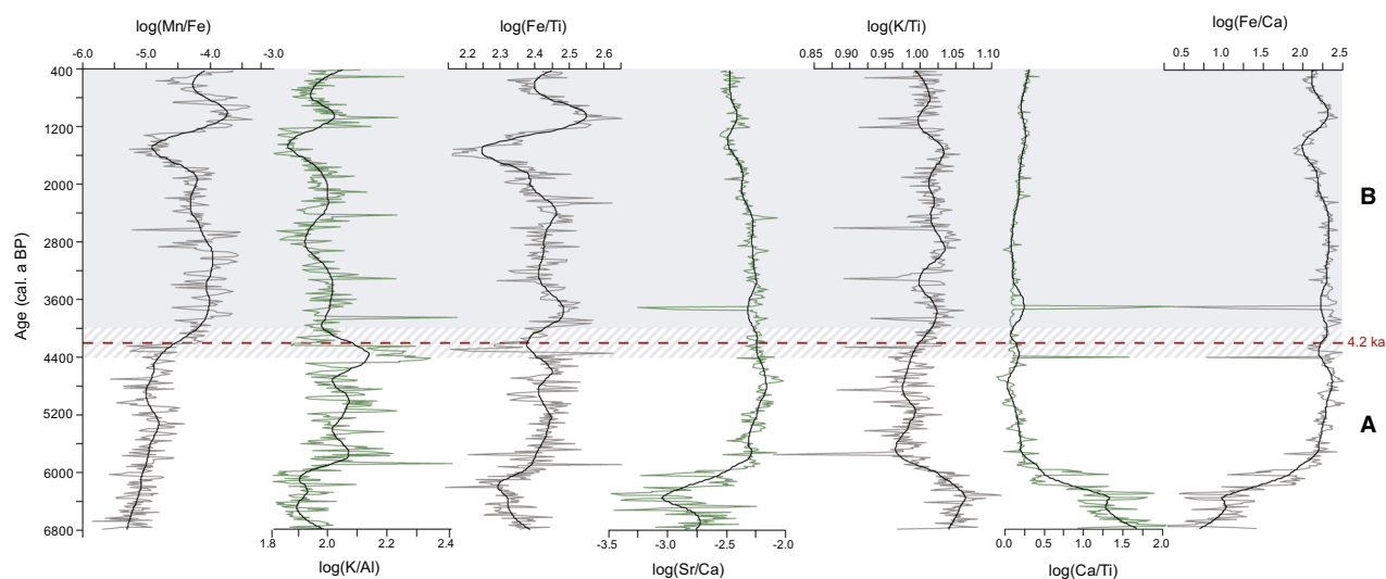
Fig. 5. Geochemical content in sediment of core HH16-1205-GC expressed as element log-ratios. Grey and green lines represent the log-ratio values and black lines represent the smoothed values after Loess regressions. Zones defined as Middle (A) and Late Holocene (B) are indicated to the right.
