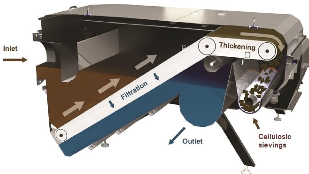
Figure 8.1 Simplified schematic representation of the working principle of microsieving, adapted from Salsnes (Norway) filter product sheet.
