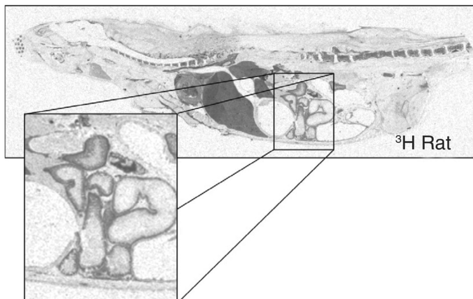
Fig. 1. Example of QWBA imaging, using ^3\text{H} -labeling in a rat. Reprinted with permission from Bioanalysis (2015) 7(5), 557–568 as agreed by Newlands Press Ltd.
