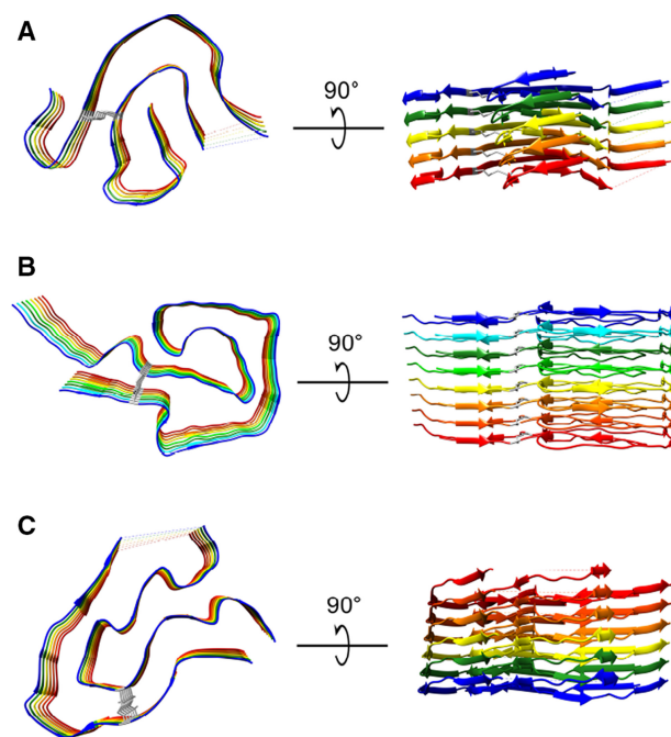
Fig. 2. Structures of amyloid fibrils from AL patients. Cryo-EM structures of (A) AL55 fibrils (PDB: 6HUD) and (B) \lambda 1 fibrils (PDB: 6IC3). (C) FOR005 fibrils in conformation A (PDB: 6Z10). In A, B and C, the different colors represent different polypeptide chains arising from V_L domains. The structures have been generated using UCSF Chimera.
