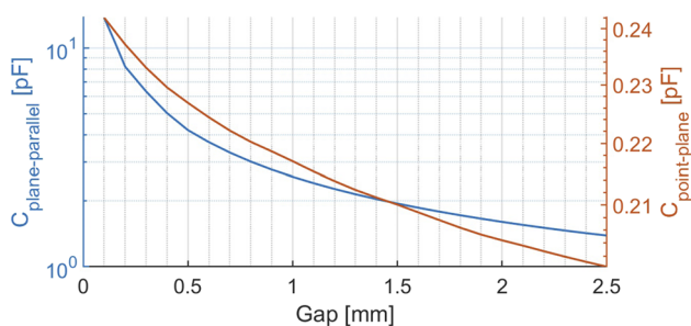
FIG. 11. Electrode capacitance for the two configurations considered.
