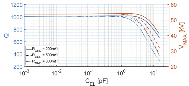
FIG. 7. Dependence of the quality factor and open-end voltage on C_{EL} and R_{GND} for Z_{0,vs} = 153 \Omega .
