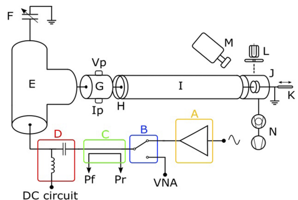
FIG. 1. IBEX schematic representation. A—solid-state amplifier, B—RF switch, C—directional coupler, D—bias tee E—9'' transmission line T section, F—tuning vacuum capacitor, G—voltage and current probes, H—vacuum feedthrough, I—high impedance transmission line section, J—test electrodes, K—linear manipulator, L—microparticle source, M—high speed camera, and N—pumping system.
