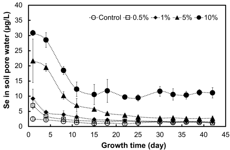
Figure 7.8. Evolution of the Se concentration in the pore water of soil amended with Se-enriched microalgae over the growth period of beans. Values are mean \pm standard deviation ( n=3 ).
