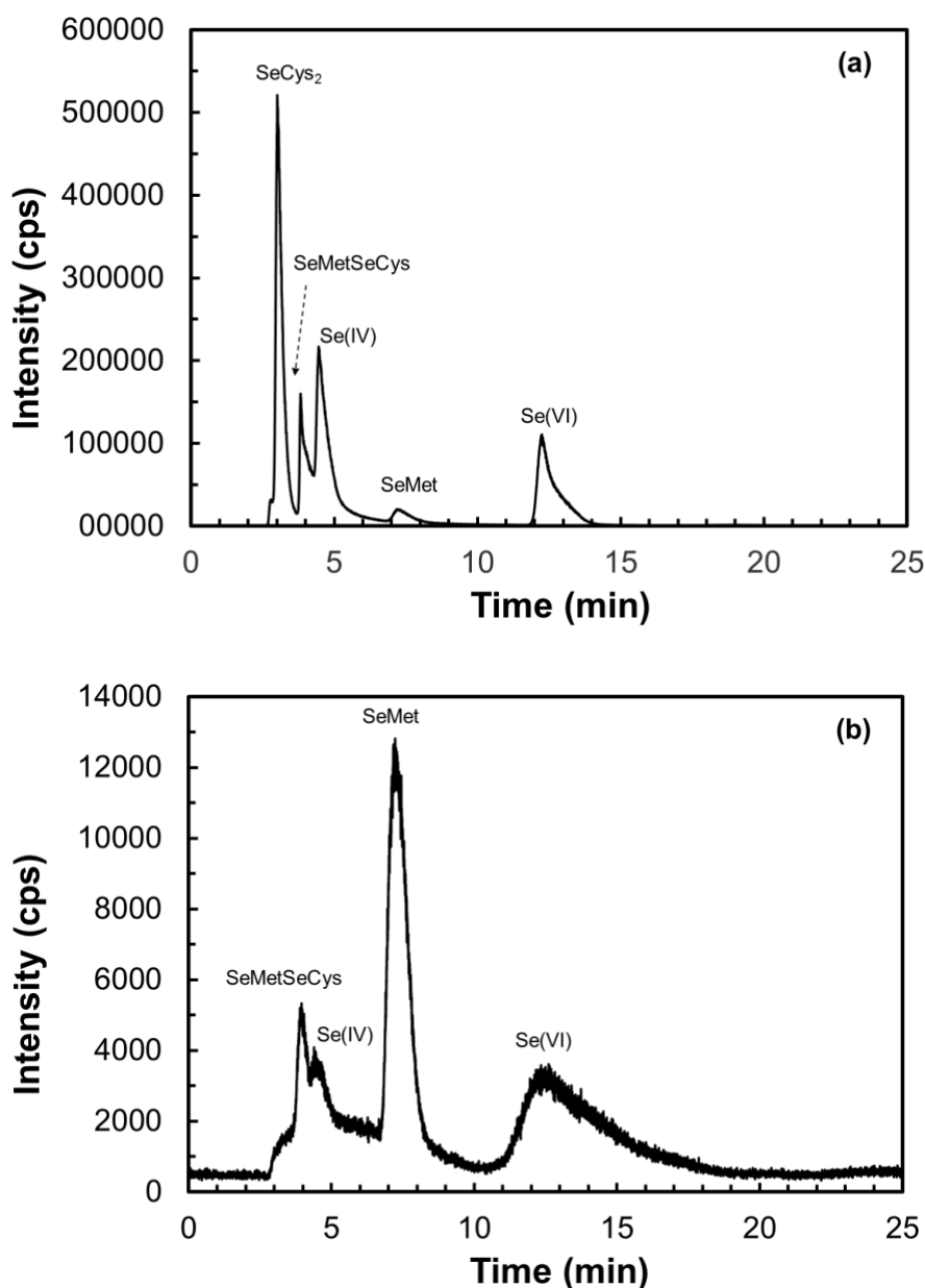
Figure 6.6. Chromatograms of Se speciation of (a) Se standard solution containing 100 µg/L of each Se species and (b) an extract of Se-enriched microalgae (diluted 20 times) grown in the HRAP-Se at the operational week 7.
