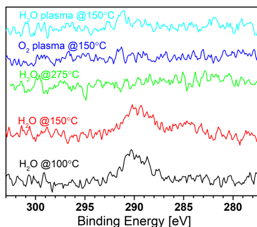
FIG. 6. The carbon details from XPS spectra of films deposited at different temperatures with different coreactants.
