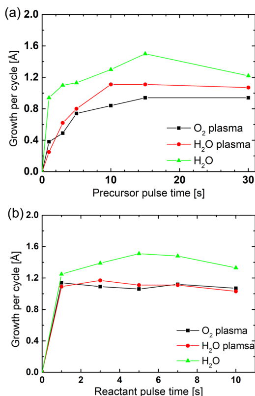
FIG. 2. Saturation curves at 150 °C: (a) 5 s coreactant pulse with different ATSB pulse time and (b) 15 s ATSB pulse with different pulse time for water, oxygen plasma, and water plasma.
