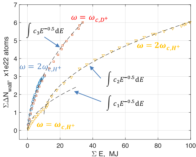
Figure 6 : Removal-integral by mass spectrometry as function of coupled energy-integral for 3 ICWC experiments on the JET-ILW at 25MHz, 100-300kW of coupled power, discharge pressure of 0.5-7.5x10 -5 mbar. Blue: D 2 -ICWC and 3.3T with 2-8 s discharges. Red: H 2 -ICWC at 25MHz and 1.65T with 2-20 s discharges. Yellow: D 2 -ICWC at 3.3T and 1.65T with 5-20 s discharges. Dashed lines: Comparative power law envelope curves.
