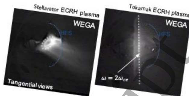
Figure 2 : He-ECRH plasma on WEGA at 28GHz (X2), 1.3 \times 10^{-4} mbar and 7.5kW launched power. Left : stellarator vacuum field of 450mT on axis with \iota/2\pi = 0.4 . Right : tokamak vacuum field of 500mT on axis with \iota/2\pi = 0 .
