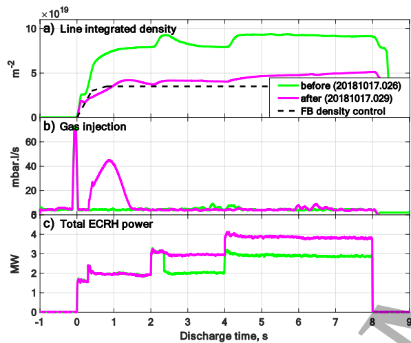
Figure 3 : Reference discharges on W7-X before (20181017.026) and after (20181017.029) application of He-ECRH conditioning. a) line integrated density and density feedback control, b) total gas injection, c) ECRH input power.
