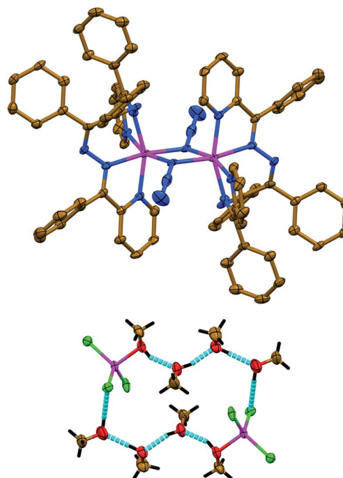
Fig. 2 (top) Crystal structure of the cationic part [\text{Zn}_2(\mu_{1,1}\text{-N}_3)_2(\text{L}^1)_2]^{2+} of 2 . Hydrogen atoms are omitted for clarity. Color code: C = gold, N = blue, Zn = magenta. (bottom) Crystal structure of the hydrogen bonded synthon of motif R_8^8(20) of the ([\text{ZnCl}_3(\text{MeOH})]_2)^{2-} \cdot 6\text{MeOH} composition, constructed from the [\text{ZnCl}_3(\text{MeOH})]^- anionic part and lattice MeOH molecules of 2 . Color code: H = black, C = gold, Cl = green, O = red, Zn = magenta.
