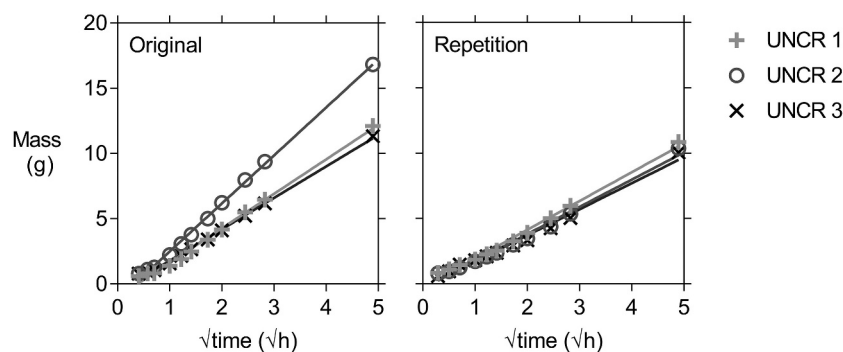
Figure 9. Comparison of the cumulative mass gain versus the square root of time for the uncracked specimens of lab 6 with the individual linear regression lines, showing a more uniform behaviour for the repeated waterproofing with aluminium tape compared to the original waterproofing with aluminium tape.
