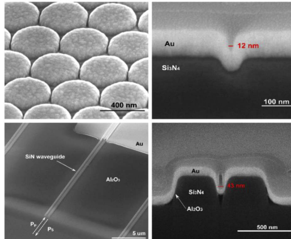
Fig. 2. (top) Gold nanodomes are free-space SERS substrate with an average gap size of 12 nm. (bottom) Waveguide-based nanoplasmonic slot waveguides have an average gap size of 43 nm.
