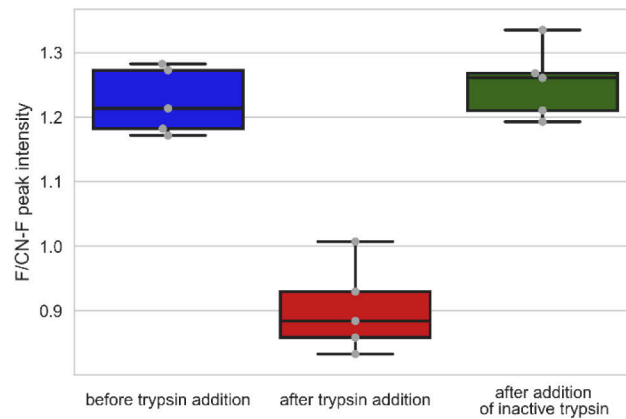
Fig. 4. F/CN-F peak intensity ratio for the trypsin cleavage experiments performed on gold nanodomes. The box plot shows that the F/CN-F peak intensity ratio decreases by 30% after trypsin addition. If no trypsin is added, or after the addition of inactive trypsin, there is no change in the F/CN-F peak intensity ratio.
