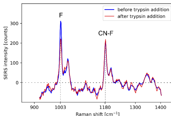
Fig. 3. SERS spectra of the peptide before and after trypsin addition, recorded on gold nanodomes. Addition of trypsin results in a decrease in the intensity of the SERS peak of phenylalanine (F) at 1003 \text{cm}^{-1} .
