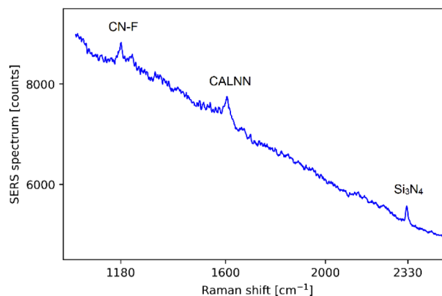
Fig. 5. Raw SERS spectrum of the trypsin peptide substrate acquired on the nanoplasmonic slot waveguide. The silicon nitride peak at 2330 cm -1 indicates that the light is guided in the waveguide, whereas the other two peaks originate from the peptide itself. The background originates predominantly from the silicon nitride waveguide.
