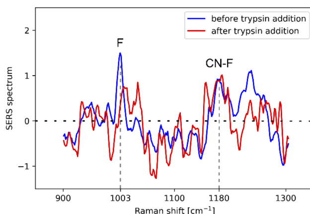
Fig. 7. SERS spectra of the peptide before and after trypsin addition acquired on nanoplasmonic slot waveguide. The decrease in the F peak at 1003\text{ cm}^{-1} indicates trypsin-mediated cleavage of the peptide. Each spectrum shown in the graph is the average of 10 background-subtracted measurements. For better visualization, the spectra were smoothed with the simple moving average with the window size of 3.
