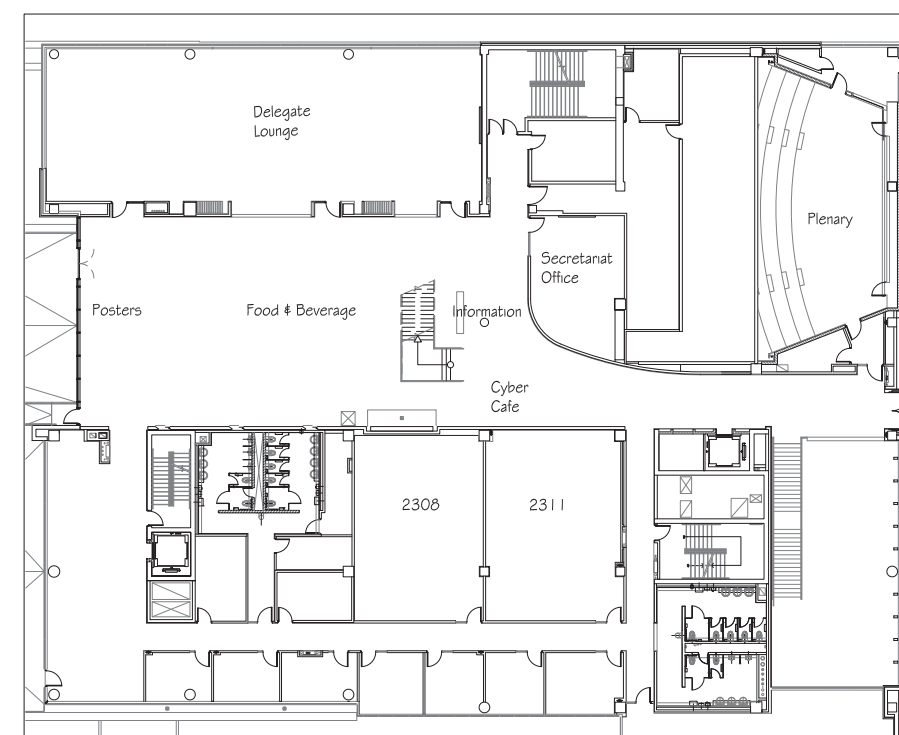
2 nd Floor
