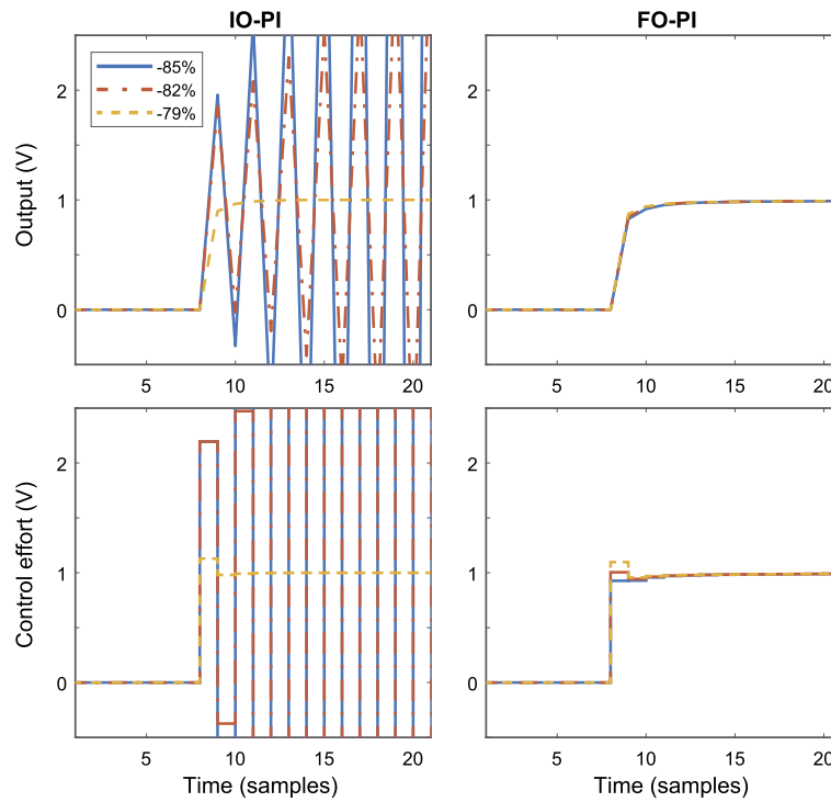
Fig. 6. The step response (up) and the control effort (down) are given for the closed-loop system for the IOPI (left) and FOPI (right) case.
