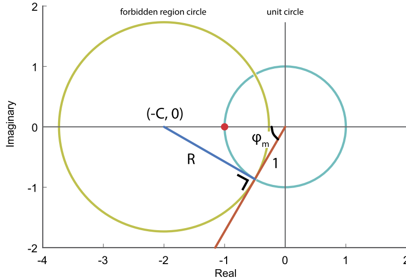
Fig. 1. Construction of the forbidden region in the Nyquist plane for the KC method.
