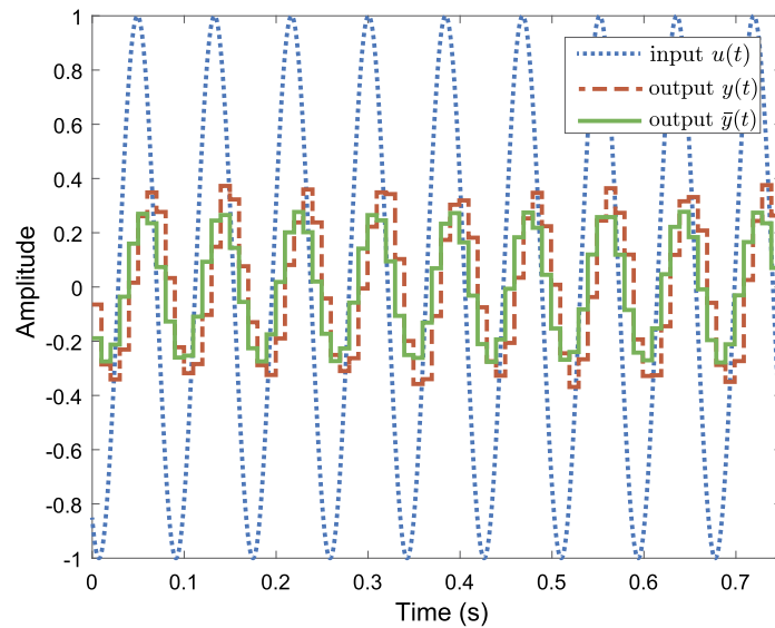
Fig. 3. The results of the sine test at \omega_{gc} : the input signal u(t) , the process output y(t) , and the signal \tilde{y}(t) to find the phase slope.
