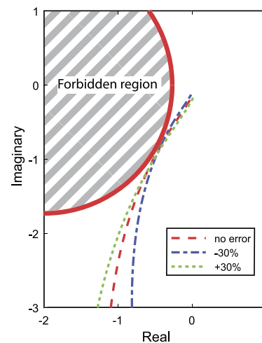
Fig. 5. The Nyquist plot of the open-loop system H_{OL}(s) with the discretized FOPI controller and variations in the process gain.
