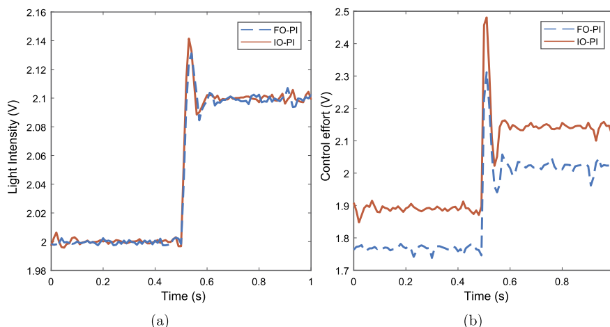
Fig. 8. Detail of the step response in zone 1. (A) the output and (B) the control effort signals around the step for the IOPI and FOPI case.
