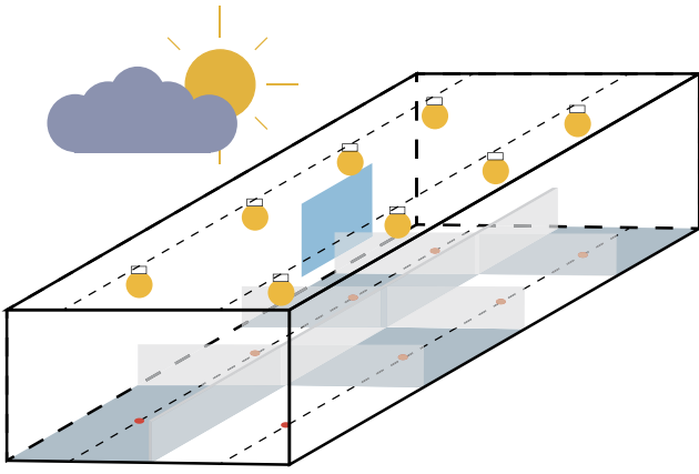
Fig. 2. Schematic representation of the light setup. The box contains eight zones that are separated by walls with a height that is smaller than the height of the box. Each zone has a lamp and a light sensor.
