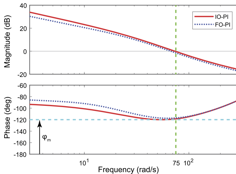
Fig. 4. The Bode plot shows the (top) magnitude and (bottom) phase of the open-loop system H_{OL}(s) with the discretized IOPI and FOPI controller.
