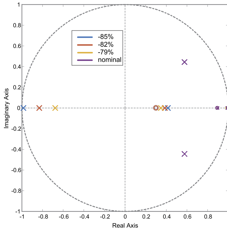
Fig. 7. The pole-zero map of the closed-loop system with the FOPI controller for process time constant variation.
