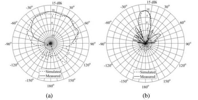
Fig. 13: Measured versus simulated, including measurement connector, radiation pattern at 38 GHz, both in the (a) E-plane ( \varphi = 0^\circ ) and (b) H-plane ( \varphi = 90^\circ ).
