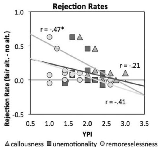
Fig. 5 Correlation with callousness, unemotionality and remorselessness with difference scores (intentionality effect: fair alternative–no alternative) in rejection rates. Delinquent data only.
