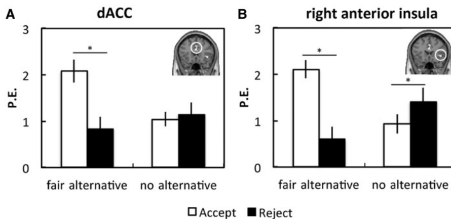
Fig. 4 Contrast values in (A) dACC and (B) right anterior insula for accepting and rejecting unfair offers in the 'fair alternative' and 'no alternative' conditions collapsed across all participants. ROI results are considered significant at a Bonferroni corrected \alpha of P < 0.008 .
