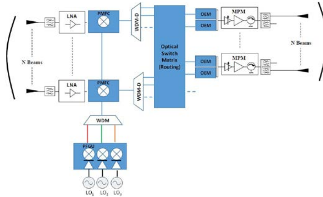
Figure 2-1 Simplified Payload Block Diagram Using Photonic Equipment
