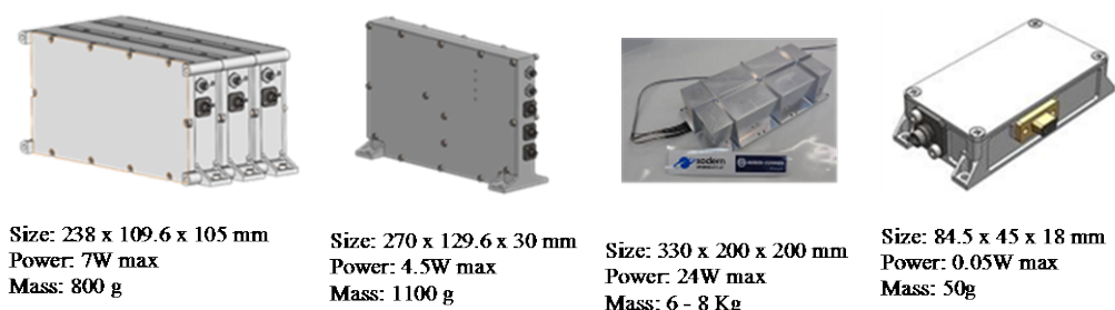
Figure 5-1 Mechanical designs of the OPTIMA modules, from left to right: PFGU, PMFC, OSM and OEM.
