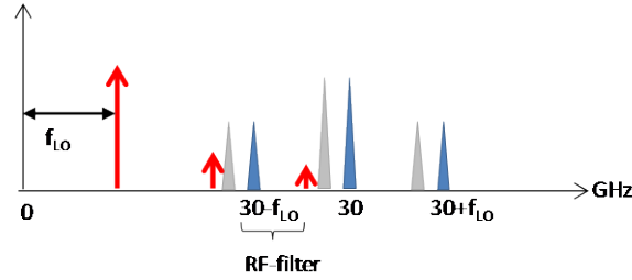
Figure 3-4 IF spectrum after optoelectronic conversion
