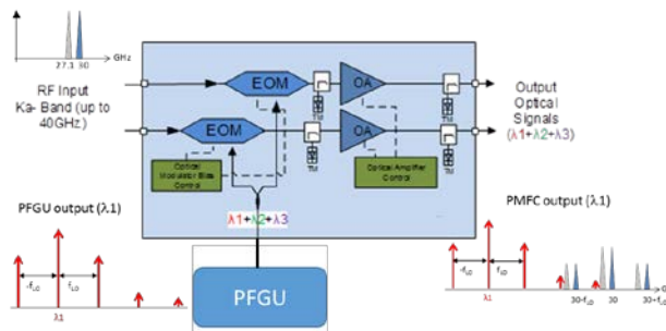
Figure 3-3 Block Diagram of Photonic Multi-frequency Converter (PMFC)
