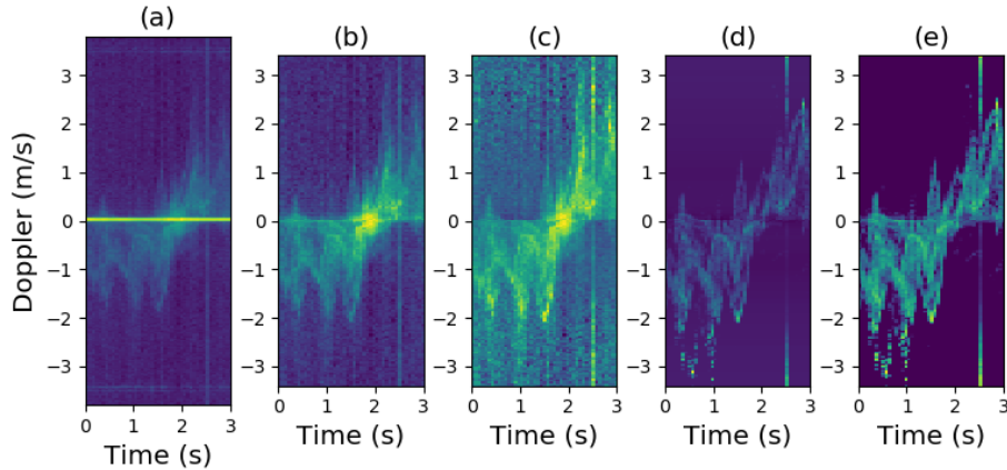
Fig. 2: A 3 second MD signature, each figure shows the results of a preprocessing step, with first (a) showing the raw signature. (b) is then obtained by removing the static channels. (c) is the normalized MD signature of (b) and still displays a lot of noise. This is then solved by applying thresholding (d) and finally the variance in the high activated areas is reduced by log scaling (e).
