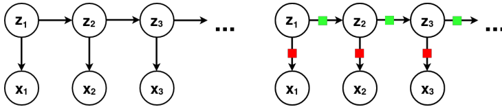
Fig. 1: Generative models of sequential data: (left) is a classical HMM. While (right) depicts a DMM. The transition (green) and emission (red) functions are both approximated using MLPs.
