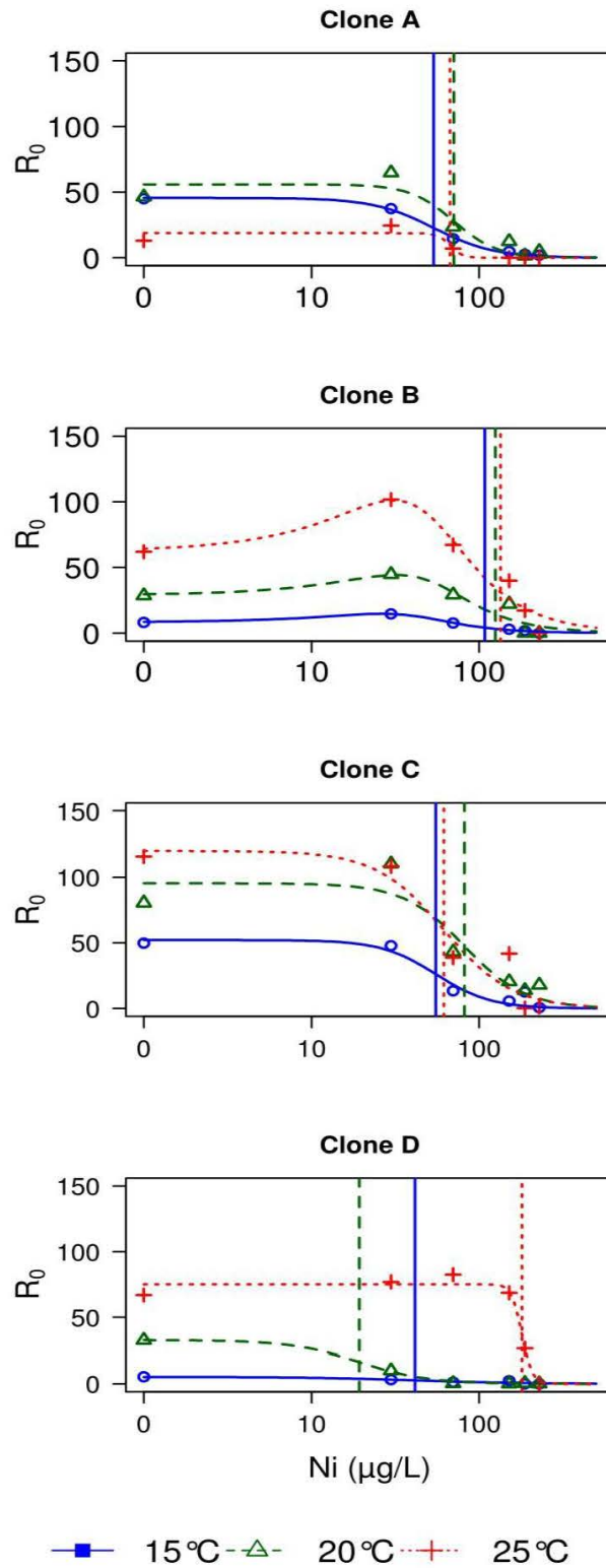
Figure 2.3. Twenty-one day concentration response curves of Ni at 15, 20 and 25°C for the four individual Daphnia magna clones calculated with the number of offspring per individual female ( R_0 ). Marker points represent average data and lines the fitted concentration response curves. Vertical lines indicate the EC50 at 15, 20 and 25°C.
