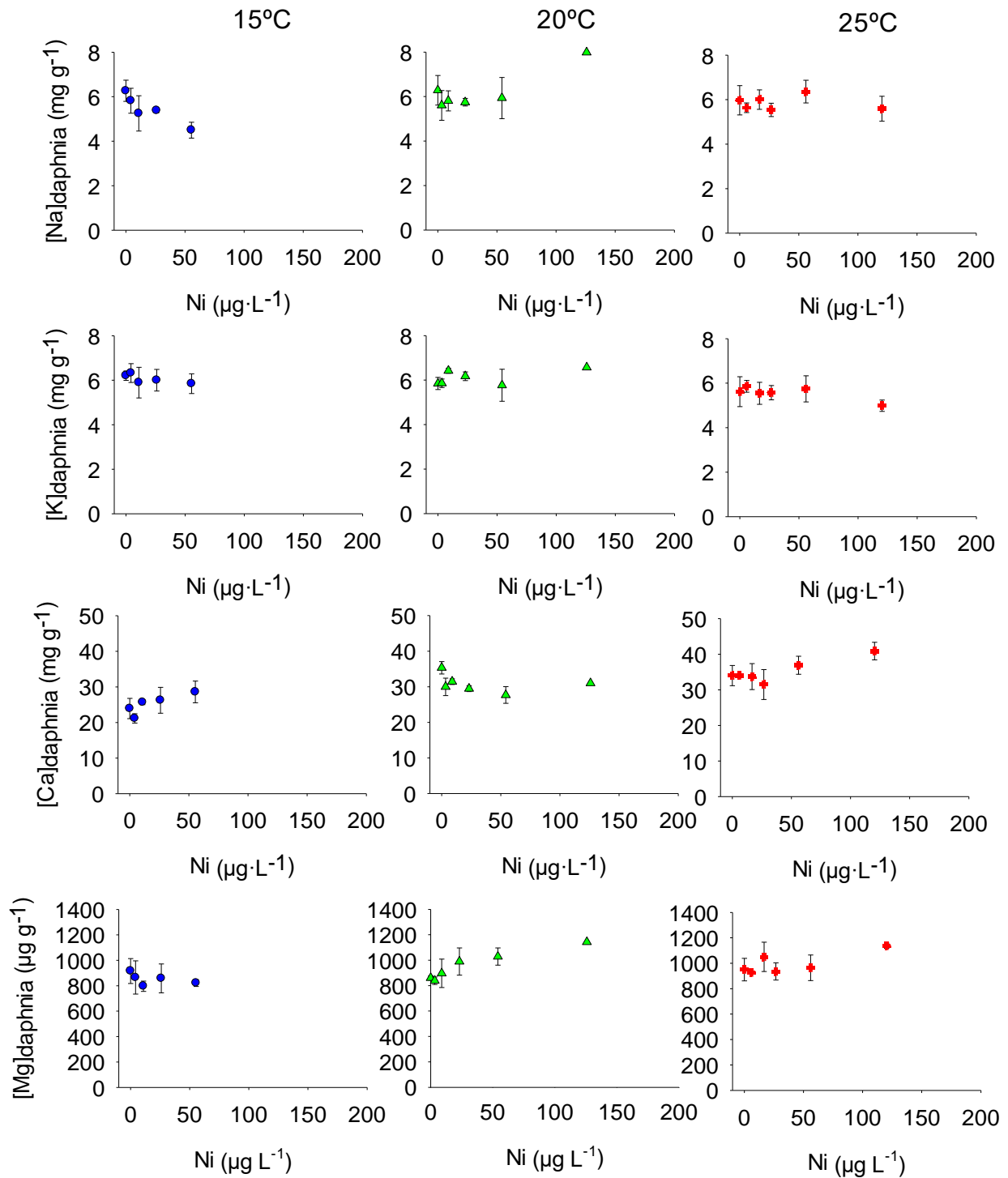
Figure 4.5. Plots of the internal Na, K, Ca and Mg concentrations in Daphnia magna (mean \pm standard deviation) on the first generation (F0) of exposure to Ni at 15, 20 and 25°C.
