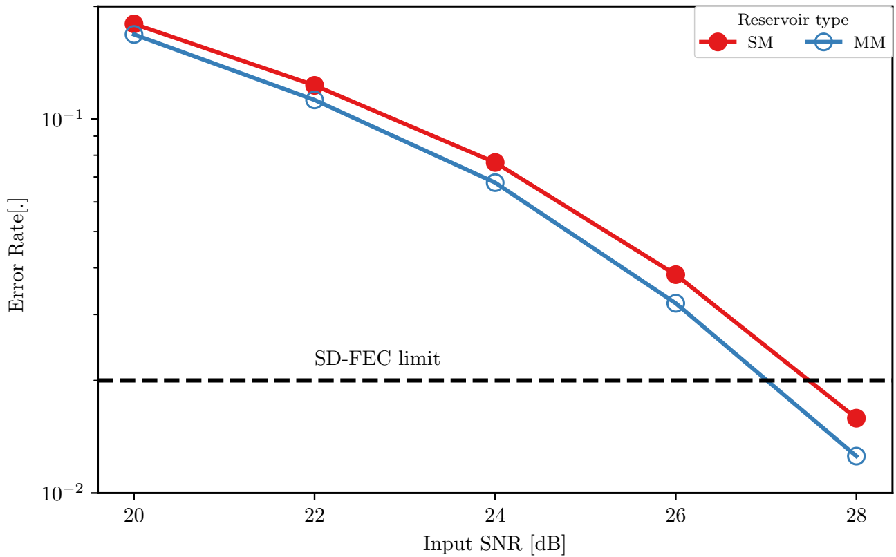
Figure 8. Error rates for single-mode and multi-mode on the 3 bit header recognition task for different values of the input SNR.
