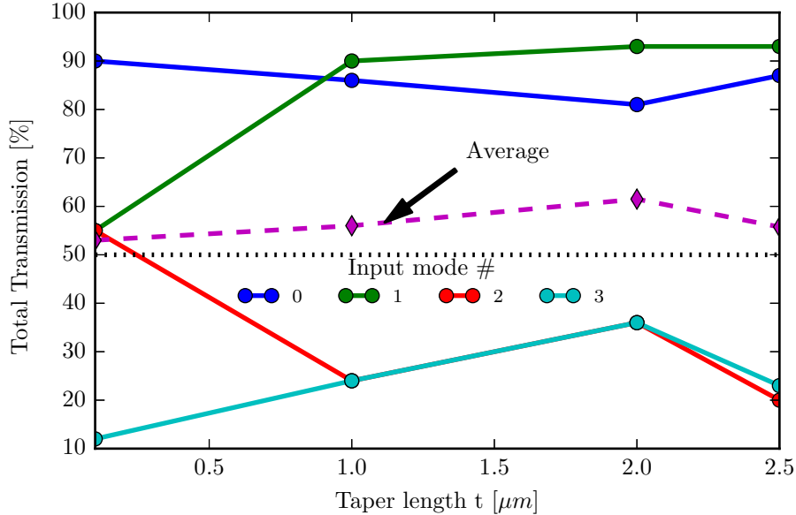
Figure 4. Total transmission (summed over all output modes) in the Y-junction combiner for different taper lengths. Results are shown for input to the upper arm of the junction consisting of the fundamental (0), 1 st , 2 nd and 3 rd order modes as well as the average transmission across all input modes. The baseline transmission of 50%, for the adiabatic single-mode Y-junction, is also indicated.
