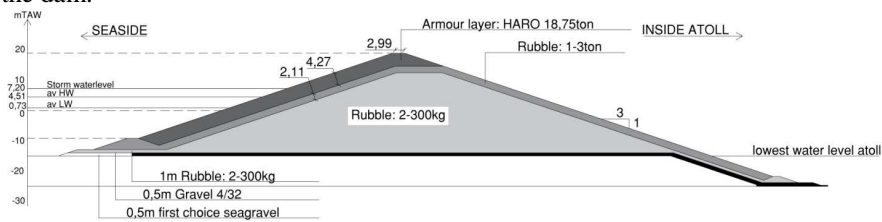
Fig. 1. Dam layout as breakwater.
