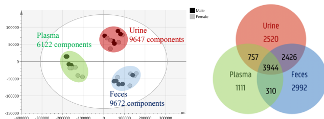
Figure 1. PCA-X score plot and Venn diagram of urine, fecal and plasma samples
