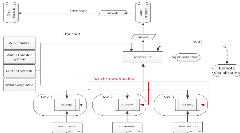
Fig. 5. Schematic of the COB Data Acquisition System
