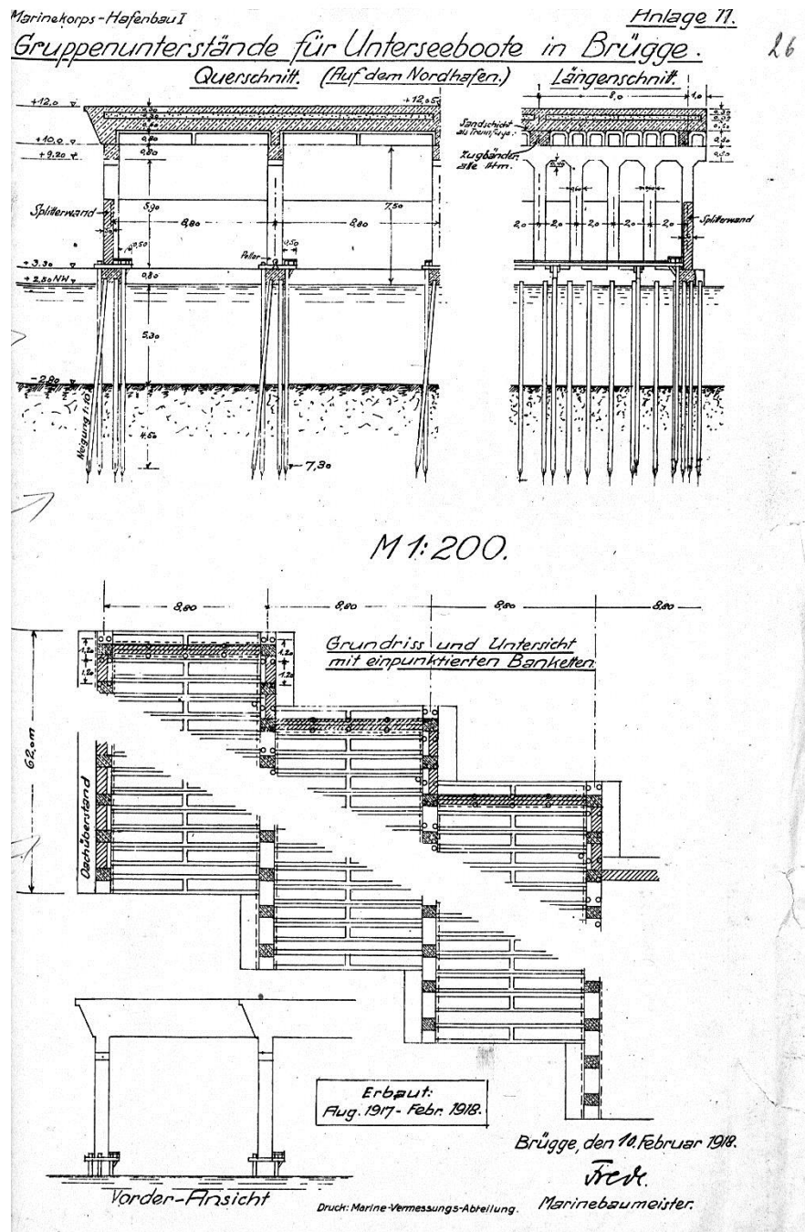
Fig. 3 – Plan, sections and facade of the Gruppenunterstand (BA-MA).
