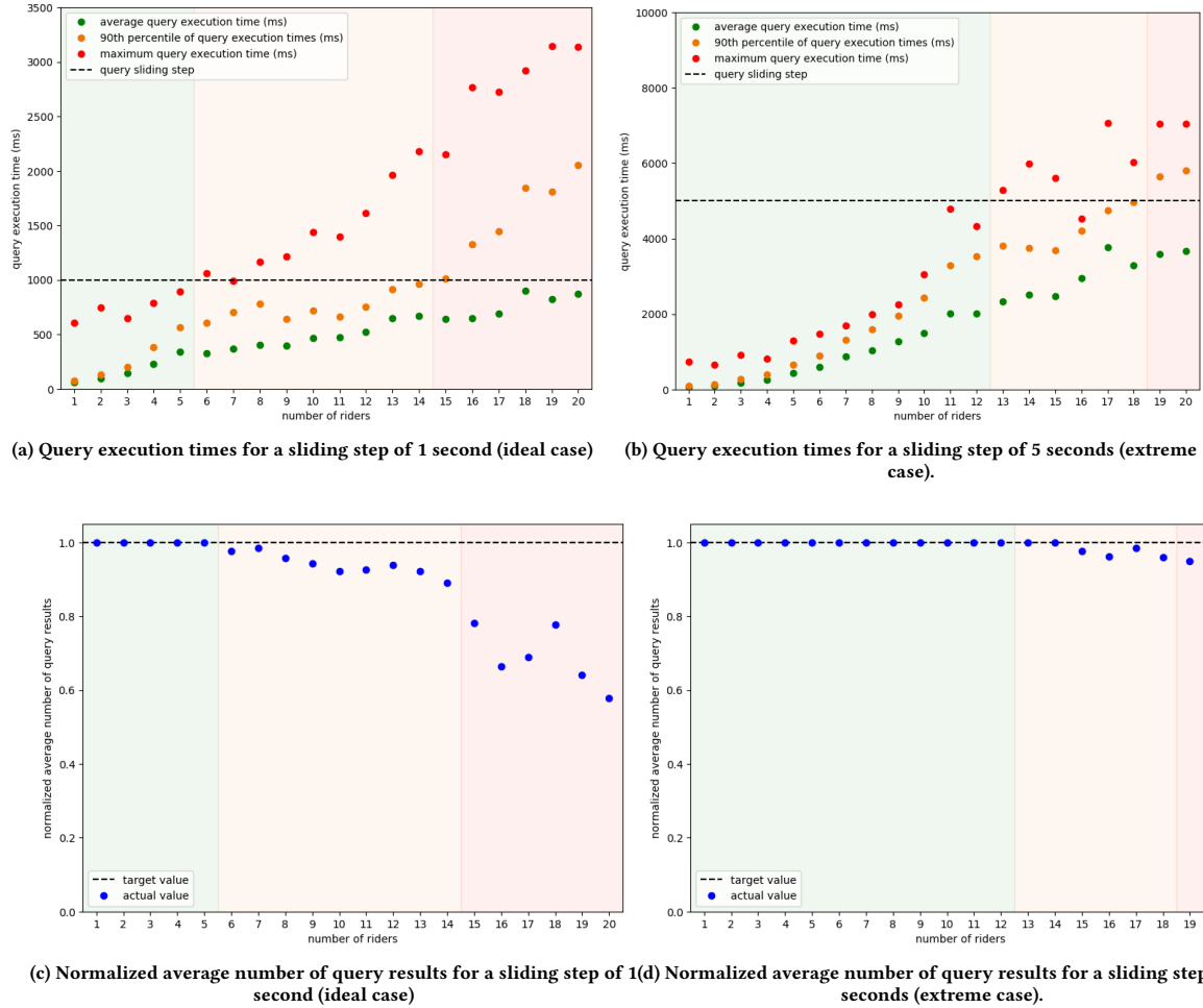
Figure 5: Query execution times and normalized average number of query results for 1 to 20 rider profiles, measured on a Raspberry Pi 3, Model B. Time between incoming heart rates is 1 second for each rider. Query window size is 10 seconds.
