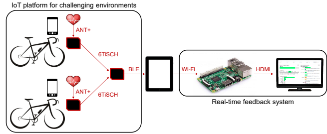
Figure 1: PoC set-up
