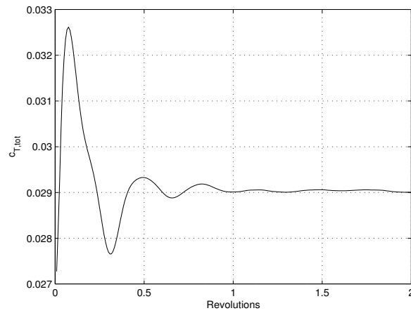
Figure 7: Total torque evolution, RO configuration.
