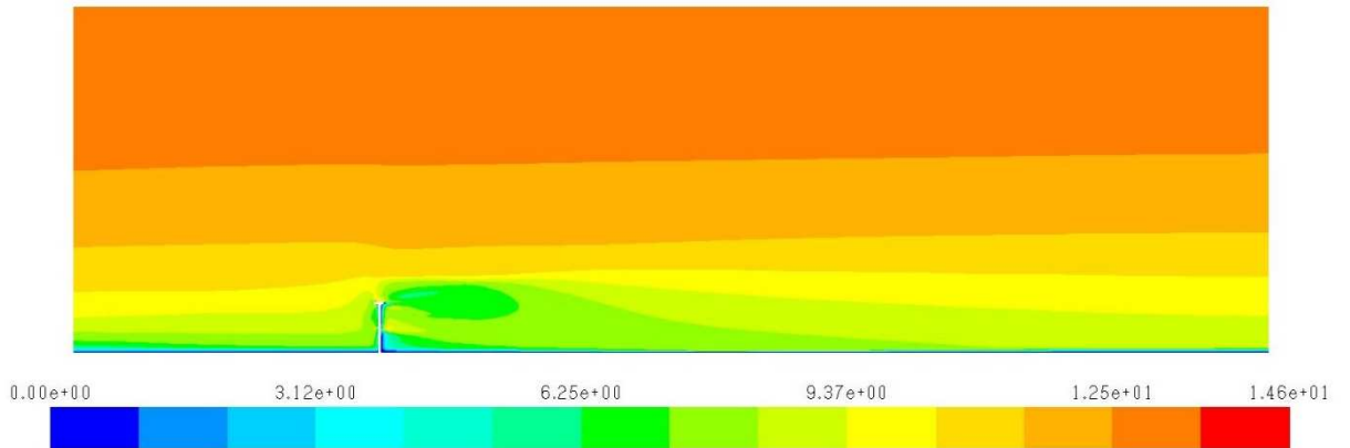
Figure 3: Contours of velocity magnitude ( \text{m/s} ) during FSI-FM simulation.
