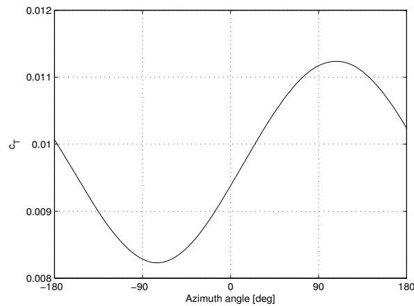
Figure 8: Single blade contribution to the torque, RO configuration.
