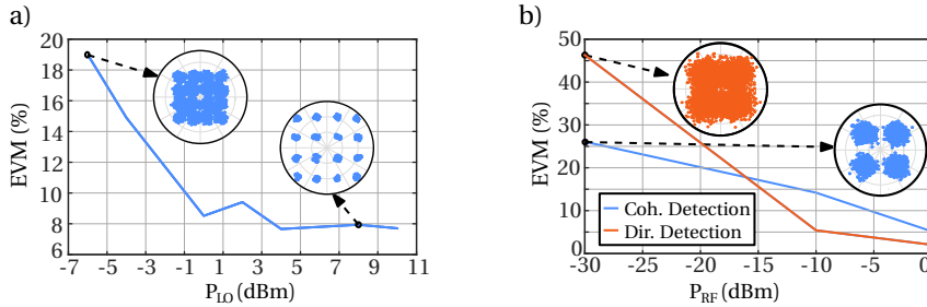
Fig. 2. a) EVM as a function of the on-chip LO power ( P_{LO} ). Representative received constellations are shown ( P_{RF} is set to 0 dBm); b) EVM for coherent vs. direct detection. At low P_{RF} coherent detection, (on-chip P_{LO} of 10 dBm), exhibits better performance.
