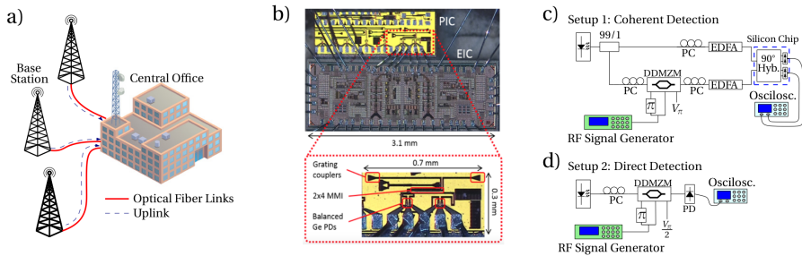
Fig. 1. a) Application of RoF transmission in the mobile access network; b) Microscope picture of the silicon photonic coherent receiver with integrated transimpedance amplifier; c) Setup 1, used for coherent reception of RoF signals; d) Setup 2, used for direct-detection reception of RoF signals.
