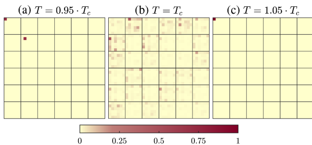
FIG. 3. Non-negative tensor elements of normalized fixed point tensors C_{1,A}^* obtained from D = 6 \text{TNR}_+ simulations of the Ising model at (a) T < T_c , (b) T = T_c , and (c) T > T_c .
