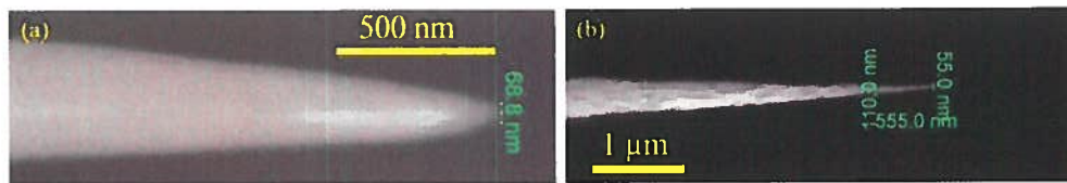
Figure 1. SEM images of fabricated silica nano-tip fiber (a) with organic overlayer, (b) without organic overlayer.
