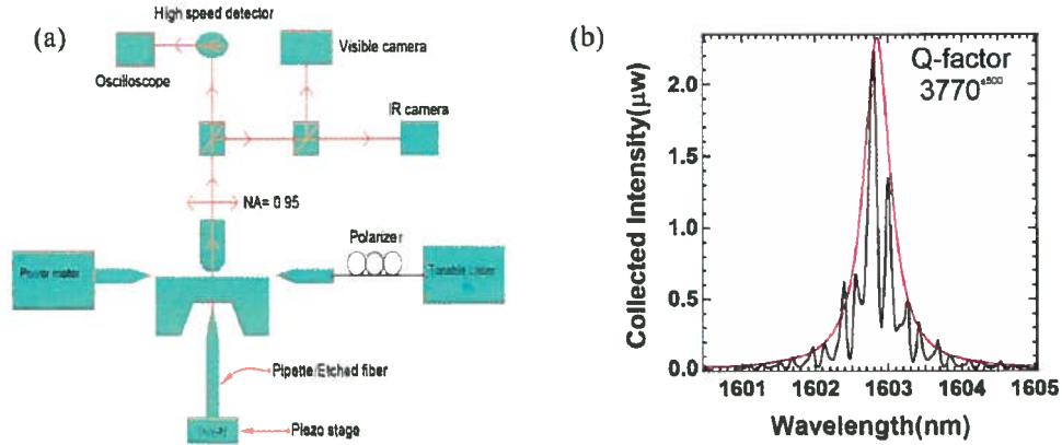
Figure 2. (a) Schematic of the experimental apparatus used for PhC mode map, (b) Transmission spectra of PhC cavity without substrate.
