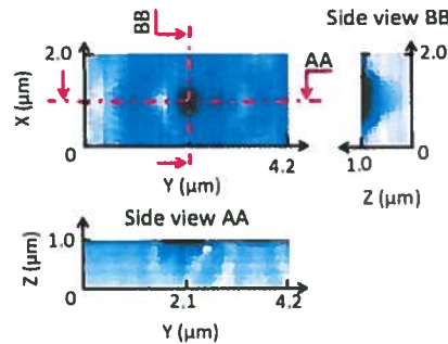
Figure 3. Three-dimensional map of the intensity variation induced by the interaction between the nano-tip fiber and the L3 cavity.
