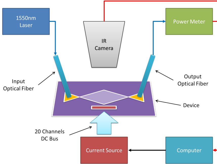
Figure 3: Measurement setup. Fibers are used for optical input and output while an IR camera is used to capture the in-circuit monitors. Heaters are driven using a 20-probe array.
