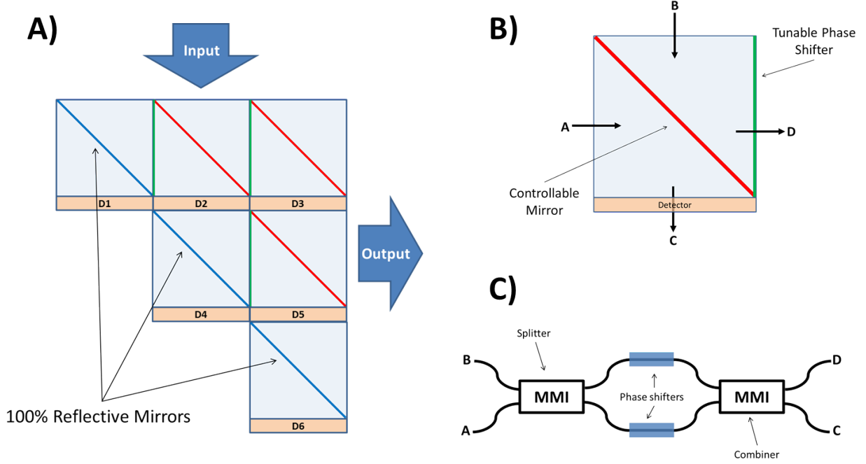
Figure 1: (a) A discrete representation of the proposed device. Diagonal red lines represents mirrors with controllable reflectivity. Vertical green lines represent controllable phase shifters. (b) Representation of an individual cell of the circuit with two inputs (a and b) and two outputs (c and d). (c) Mach-Zehnder implementation of the building block cell with two inputs (a and b) and two outputs (c and d).
