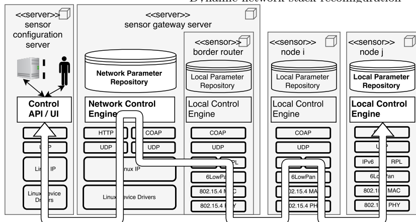
Fig. 3: The communication flow between the different entities in the architecture. The white boxes with bold text depict the active components in this example.
