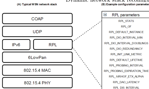
Fig. 1: (A) IPv6 compliant network stack available in TinyOS, Contiki and RIOT. (B) possible configuration parameters to fine-tune the RPL routing protocol.
