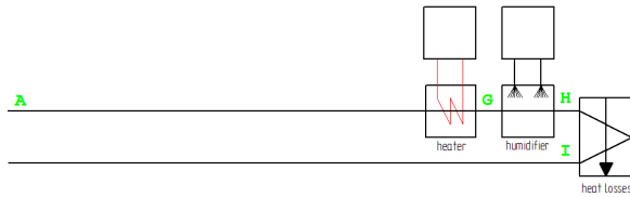
Fig. 5. Open-cycle dryer
