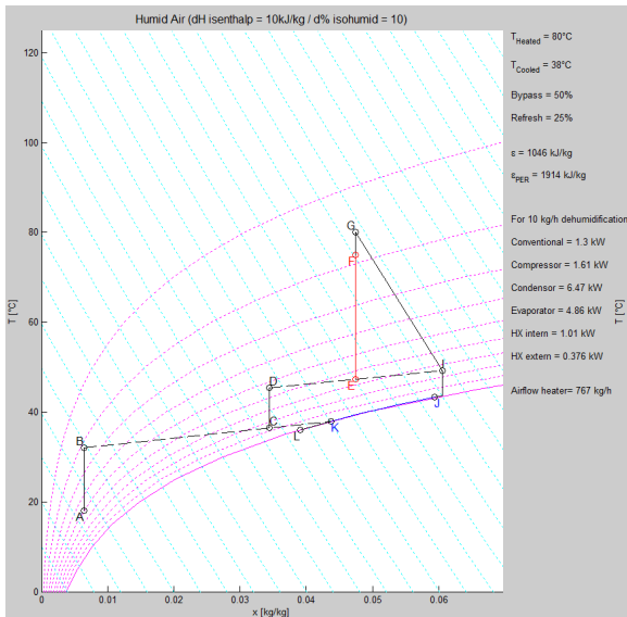
Fig. 18. Example of the simulation output for heat pump dryer with evaporator bypass, external heat exchanger and recirculation
