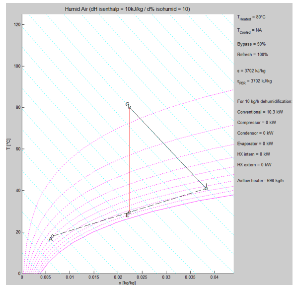
Fig. 8. Example of the simulation output for a partially closed-cycle dryer
