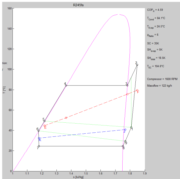
Fig. 25. Example of simulation output for a heat pump dryer with evaporator bypass, internal/external heat exchangers, recirculation, SLHX and subcooler (heat pump cycle)
