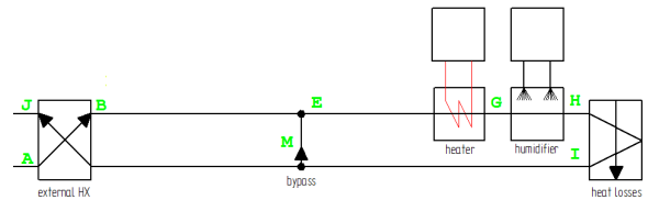
Fig. 9. Partially closed-cycle dryer with heat exchanger
