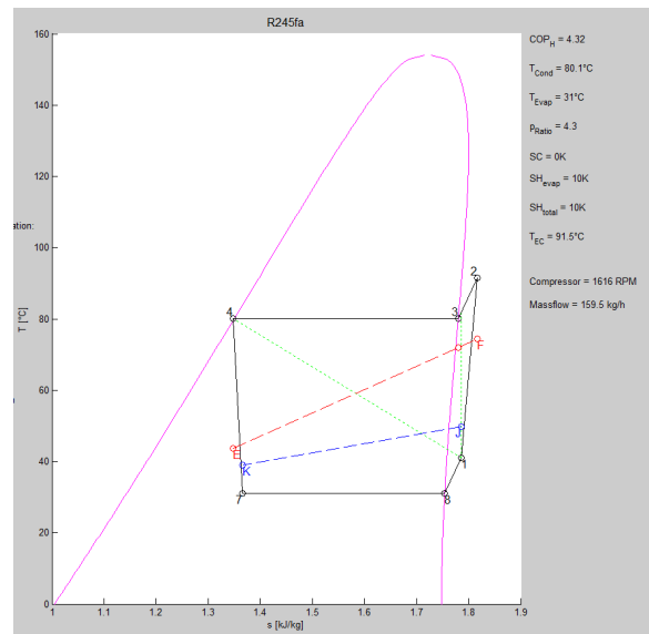
Fig. 16. Example of the simulation output for heat pump dryer with evaporator bypass, external heat exchanger and recirculation (heat pump cycle)
