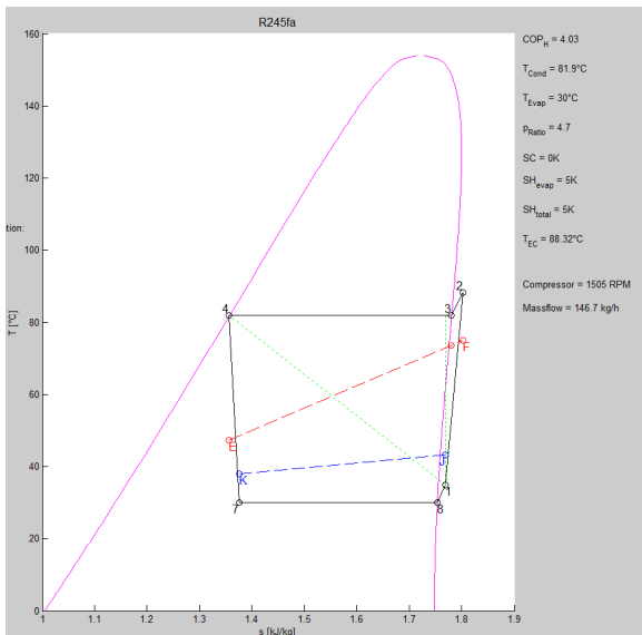
Fig. 19. Example of the simulation output for heat pump dryer with evaporator bypass, external heat exchanger and recirculation (heat pump cycle)
