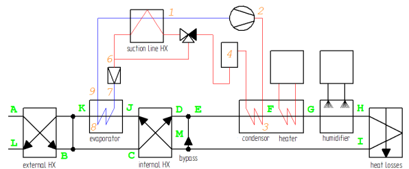
Fig. 20. Test bench simplified schematics
