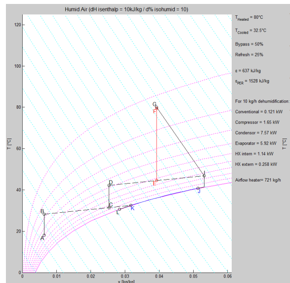
Fig. 24. Example of simulation output for a heat pump dryer with evaporator bypass, internal/external heat exchangers, recirculation, SLHX and subcooler
