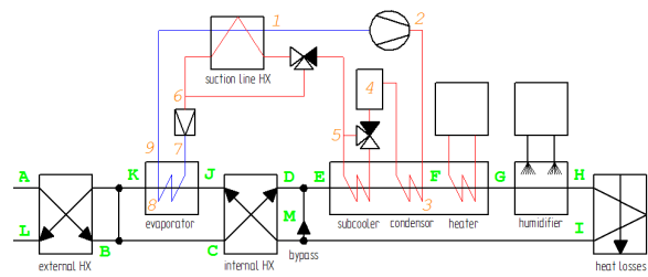
Fig. 23. Heat pump dryer with evaporator bypass, internal/external heat exchangers, recirculation, SLHX and subcooler
