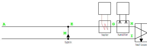
Fig. 7. Partially closed-cycle dryer
