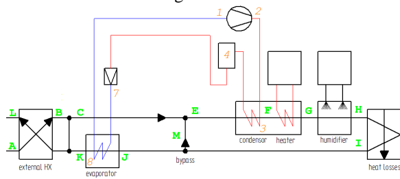
Fig. 14. Heat pump dryer with evaporator bypass, external heat exchanger and recirculation
