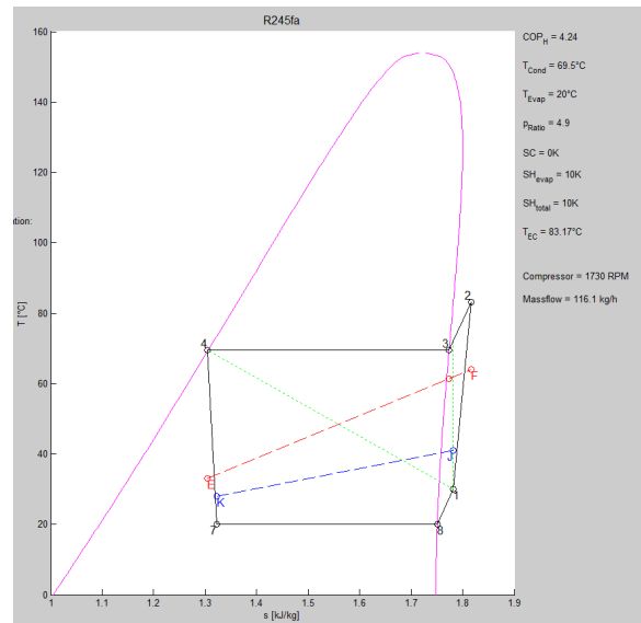
Fig. 13. Example of the simulation output for heat pump dryer with evaporator bypass and external heat exchanger (heat pump cycle)
