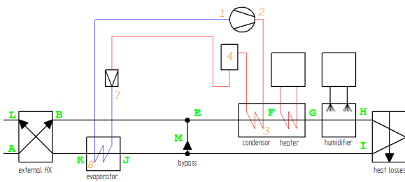
Fig. 11. Heat pump dryer with evaporator bypass and external heat exchanger
