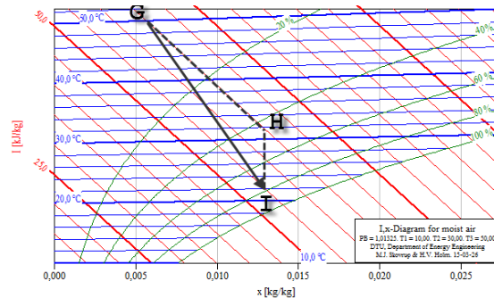
Fig. 4. Drying process reproduction
