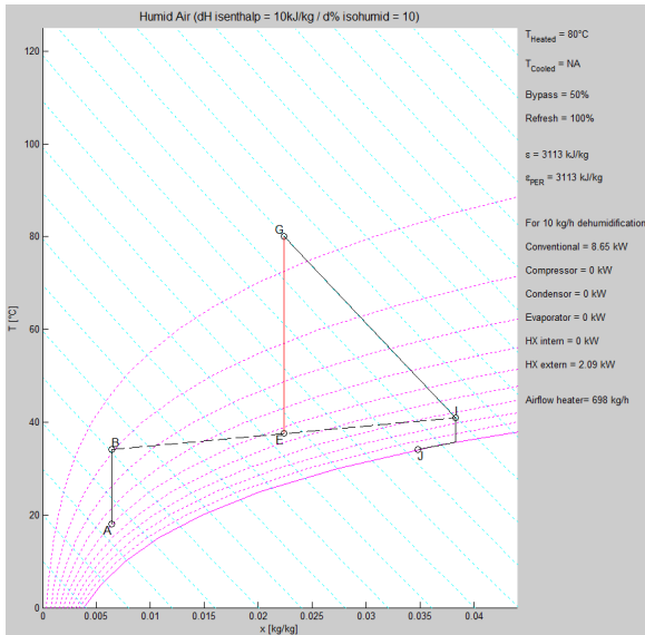
Fig. 10. Example of the simulation output for a partially closed-cycle dryer with heat exchanger
