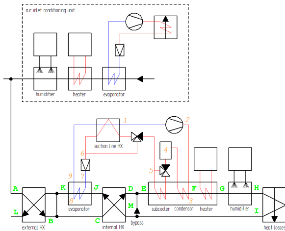
Fig. 2. Test bench simplified schematics
