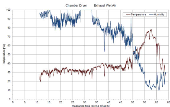
Fig. 3. Drying process reproduction
