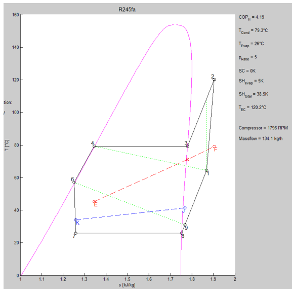
Fig. 22. Example of simulation output for a heat pump dryer with evaporator bypass, internal/external heat exchangers, recirculation and SLHX (heat pump cycle)
