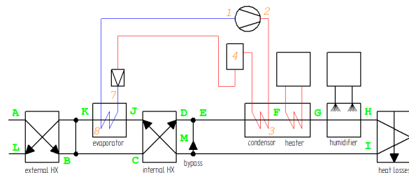
Fig. 17. Heat pump dryer with evaporator bypass, internal/external heat exchangers and recirculation
