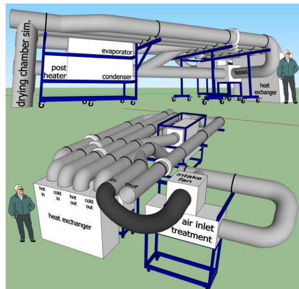
Fig. 1. Test bench design
