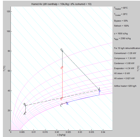
Fig. 12. Example of the simulation output for heat pump dryer with evaporator bypass, external heat exchanger and recirculation
