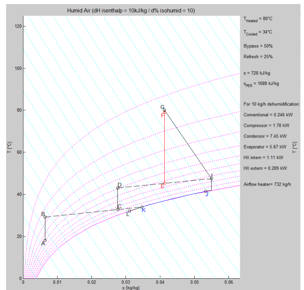
Fig. 21. Example of the simulation output for heat pump dryer with evaporator bypass, external heat exchanger and recirculation
