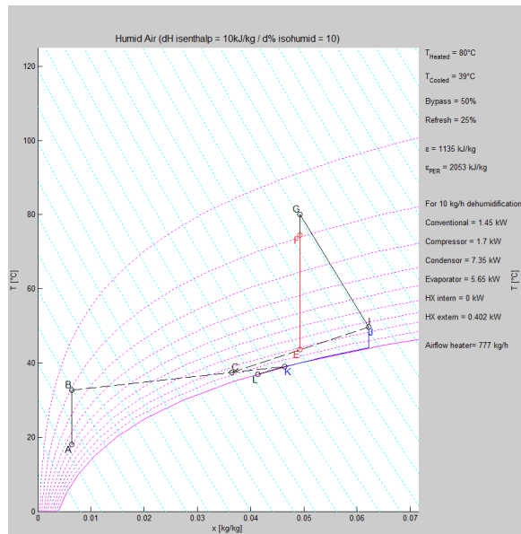
Fig. 15. Example of the simulation output for heat pump dryer with evaporator bypass, external heat exchanger and recirculation
