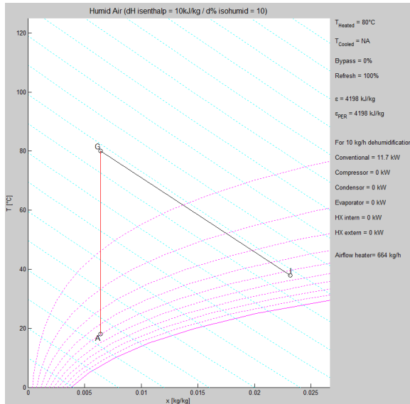
Fig. 6. Example of the simulation output for an open-cycle dryer
