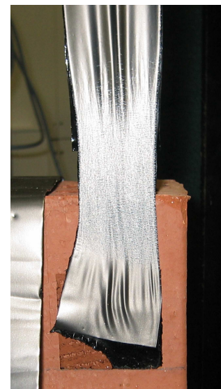
Fig.6 Adhesive failure
