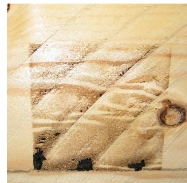
Fig.3 Adhesive failure
