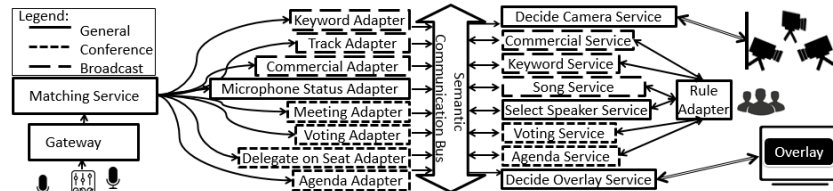
Figure 1. Mapping of the constructed Services & Adapters to MASSIF.
