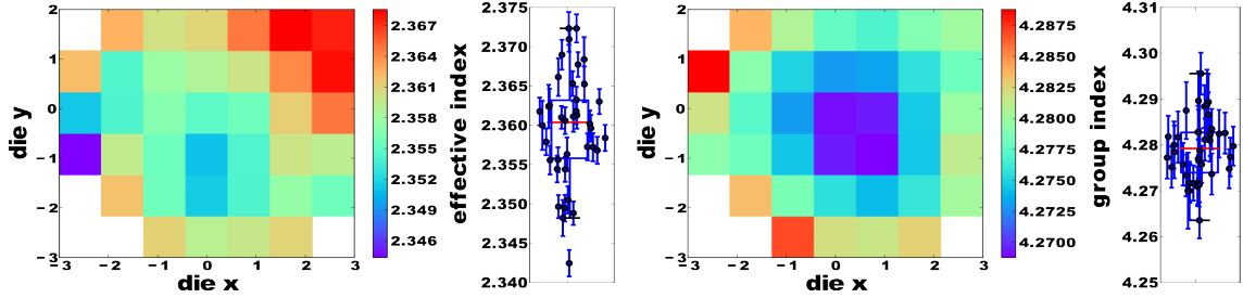
Fig. 4: Wafer statistics and map at 1550 nm (a) n_{eff} and (b) n_g
