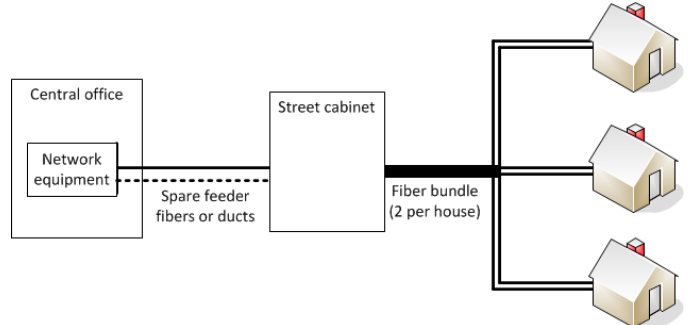
Figure 2: Overview of the impact of fibre unbundling on the network deployment cost
