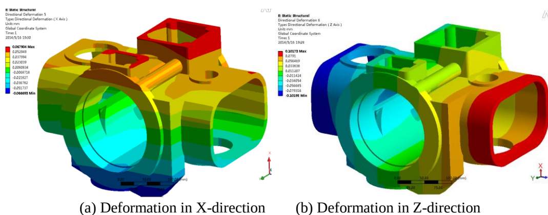
Figure 8. Deformation of the casing.
