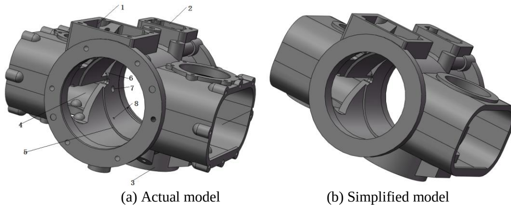
1—suction channel 2—oil path 3—exhaust channel 4—star wheel chamber 5—enclosed screw spiral 6—exhaust orifice 7—high pressure gas leak hole 8—oil injection hole
