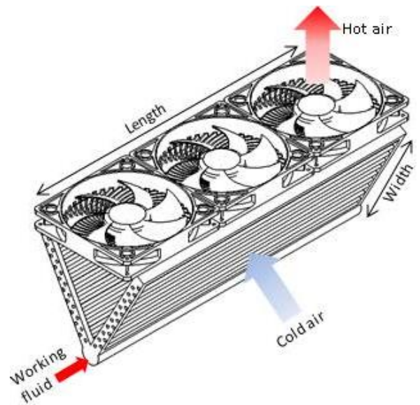
Figure 1 Condenser geometry
