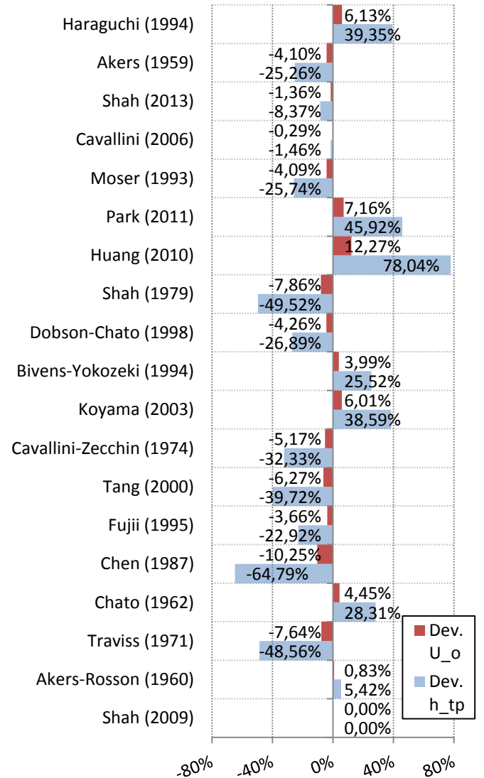
Figure 2 Deviation of U_o with respect to the deviation of h_{tp}
