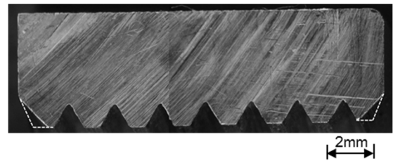
Fig. 2 Incomplete threads at nut ends
