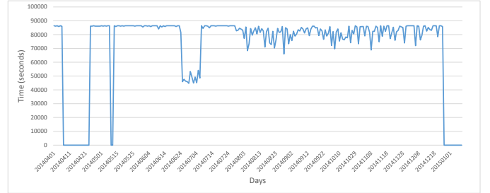
Figure 5: The running moving average of visits duration.
