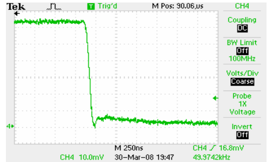
Fig.11 Turn-off current waveform IGBT in leg.
