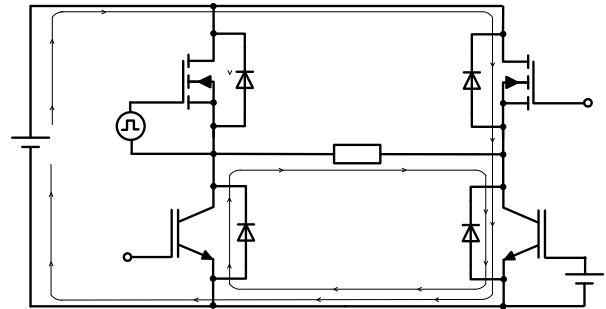
Fig.1 IGBT and MOSFET Bridge circuit.
