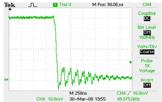
Fig. 10 Turn-off current waveform MOSFET&IGBT in leg.
