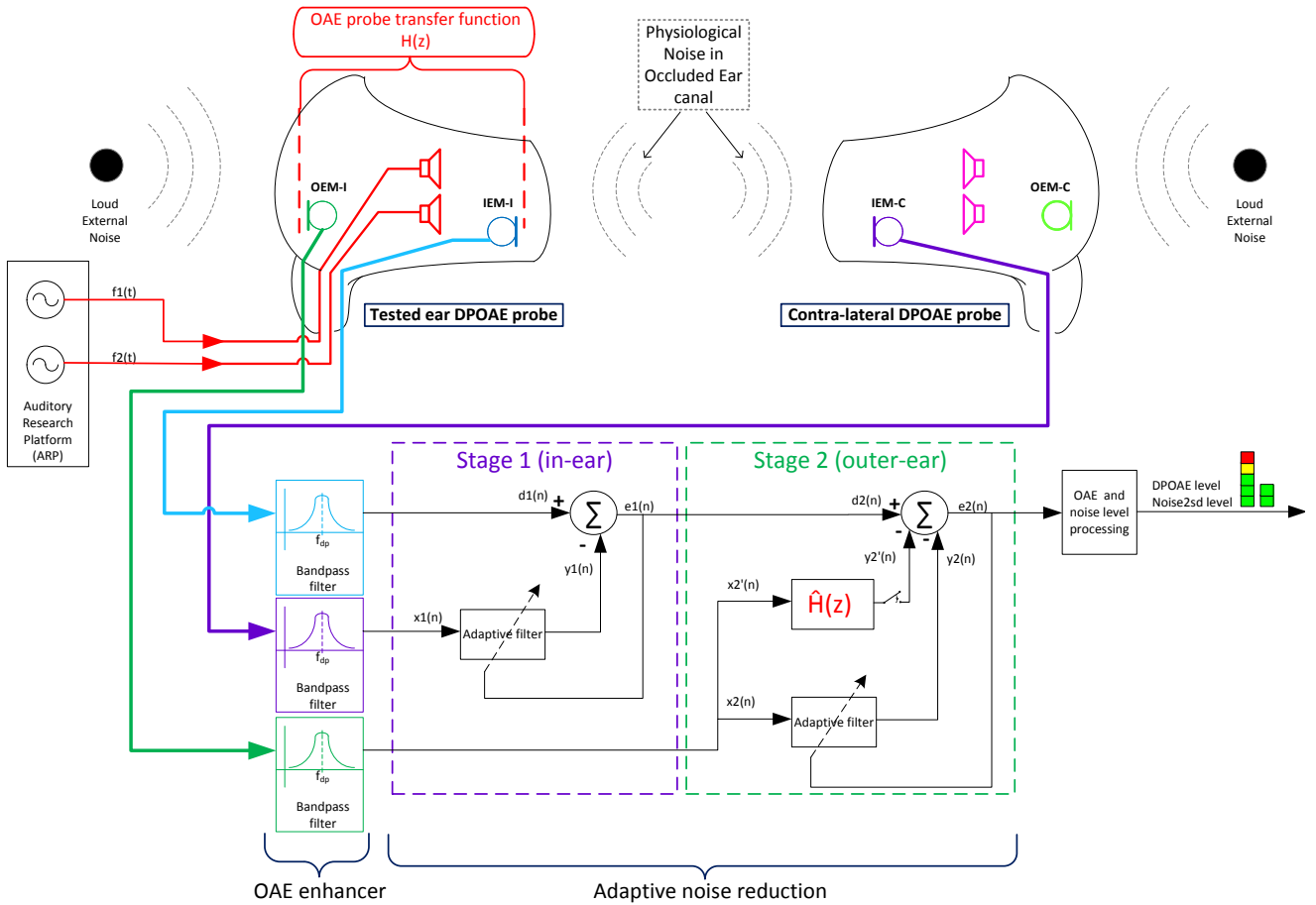
Figure 5: Block diagram of the proposed Adaptive Noise Reduction algorithm
