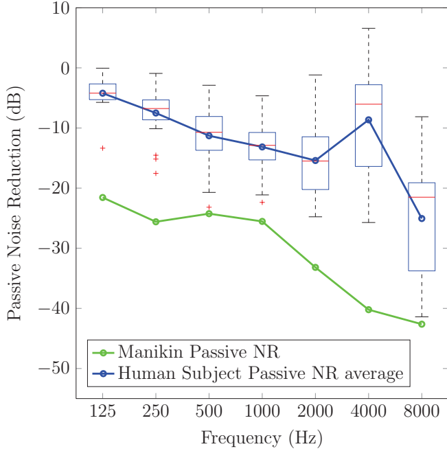
Figure 10: Intersubject Passive Noise Reduction (NR) of the roll-down foam tip used for the passive sound isolation of the developed OAE probe.
