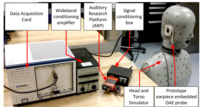
Figure 2: DPOAE data acquisition system (minimal setup shown): The Auditory Research Platform (ARP) system is connected to the signal conditioning box providing the signals to the data acquisition card and into which the prototype earpieces-embedded OAE probes are connected.
