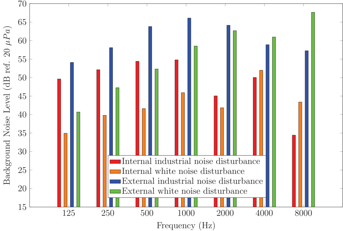
Figure 6: External microphone and internal microphone background noise disturbance level. The level of industrial noise in a first sound capture and white noise in a second sound capture in dB(SPL) are shown for the external microphone (70 dB(A) noise disturbance) and internal microphone measured per octave bands on a typical test subject while testing.
