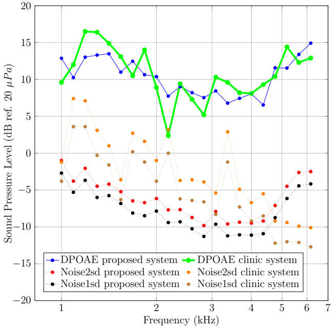
Figure 7: Typical DPgram output by the proposed system in quiet test conditions compared to the clinical system.
