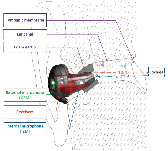
Figure 1: Earpiece-embedded OAE probe. G_1(z) and G_2(z) represent the acoustic path between the internal microphone and each miniature receiver. Receiver R1 generates the pure-tone stimulus with frequency f_1 and receiver R2 the second pure-tone stimulus f_2 .
