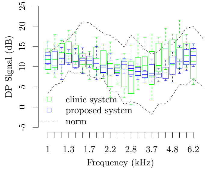
Figure 8: Box-and-whisker plot of DPOAE amplitude as a function of frequency as measured by the clinical system and the proposed system. The range of DPOAE amplitudes obtained for young, normal-hearing adults by [12] has been added as a reference ('norm').
