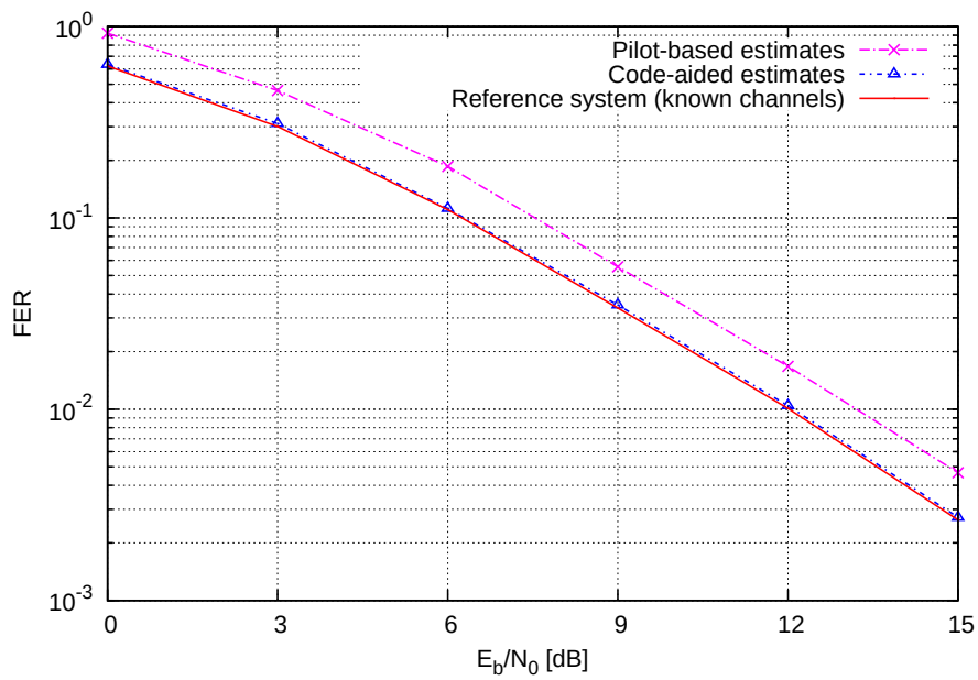
Figure 5 FER performance of a two-way QF system, in which the unknown channel parameters are estimated using different estimation techniques, as function of the E_b/N_0 ratio for a relay position that is uniformly distributed on a line connecting T_0 and T_1 .
