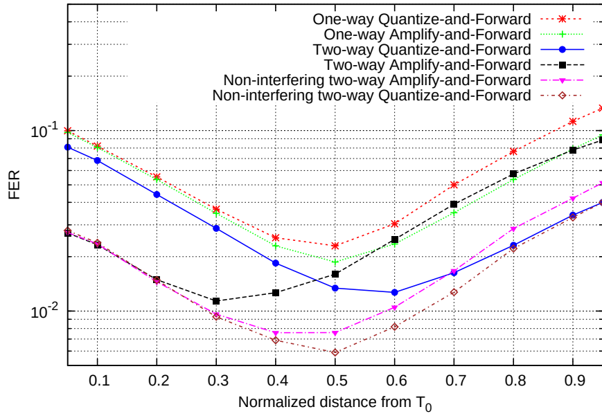
Figure 4 FER of a one-way and a two-way QF and AF protocol, along with the FER of a non-interfering two-way QF and AF system as function of the normalized distance between transmitting terminal and relay for a fixed E_b/N_0 ratio of 9dB.
