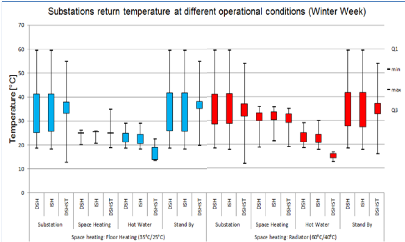
Fig.4 Return temperatures at different operational conditions radiator and floor heating for space
