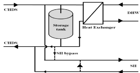
Fig. 2 Scheme of the direct system with storage tank [10].
