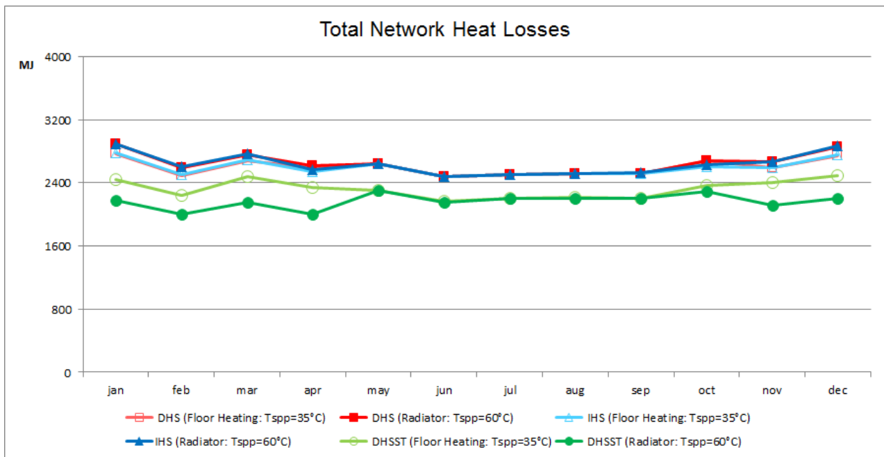
Fig. 6 Heat losses in the distribution network
