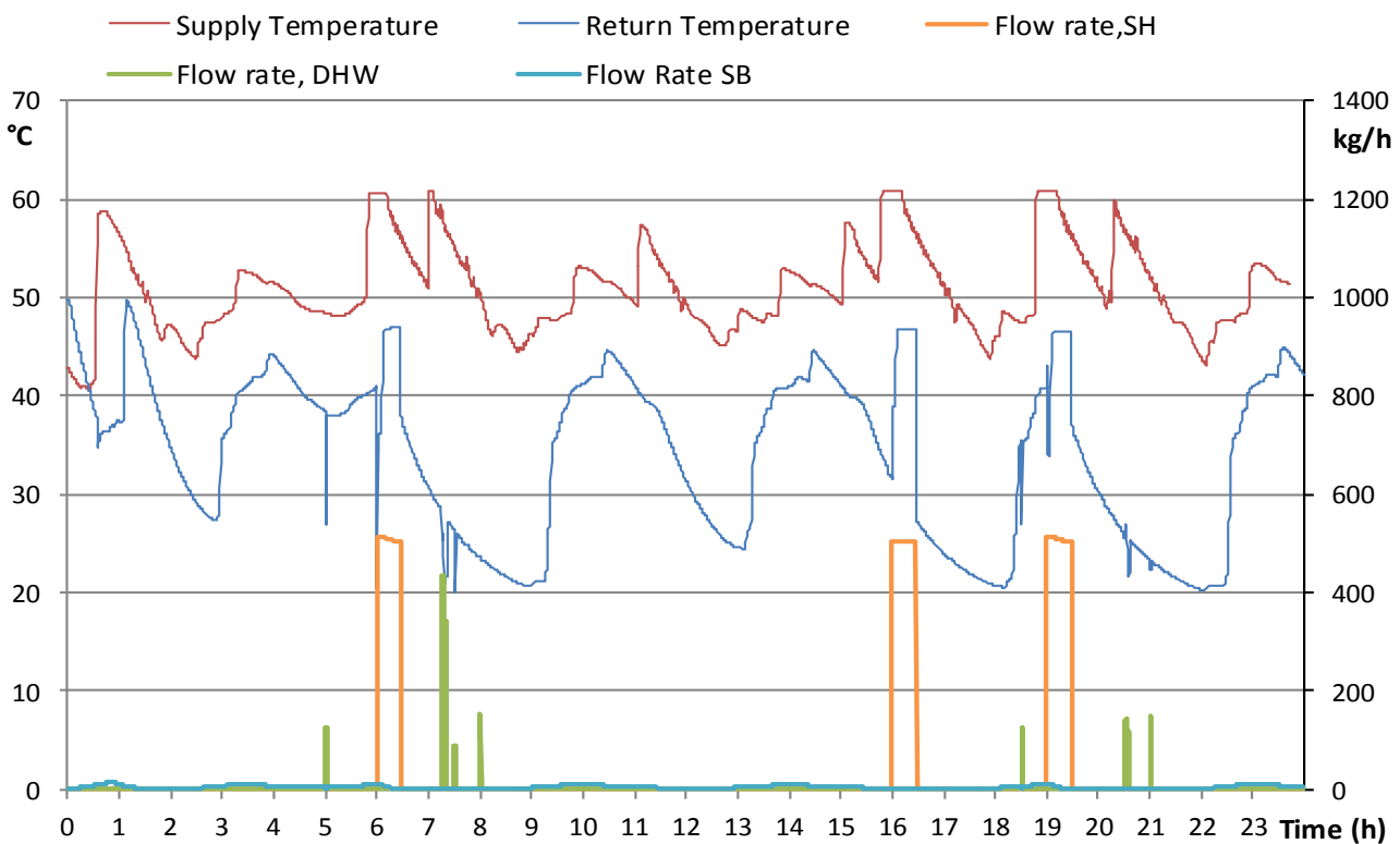
Fig.3 Supply and Return temperature at the substation of one dwellings with DHS substation
