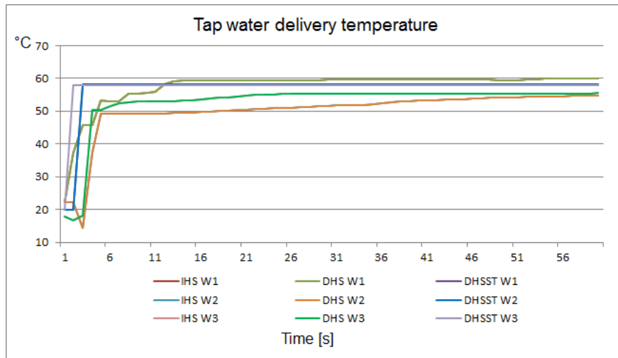
Fig. 7 Substations Tap water deliveries temperature
