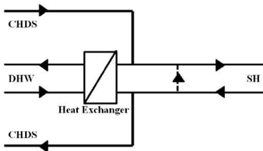
Fig. 1 Scheme of the direct system [9].
