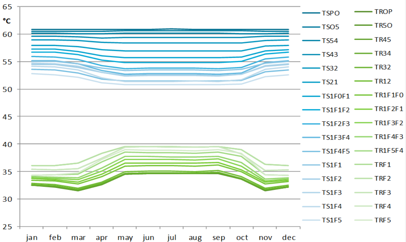
Fig. 5 Temperatures in Supply and Return pipes from main pipes (in dark) to substation connections (light)
