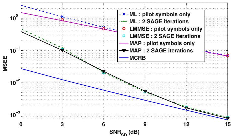
Figure 1 The MSEE related to h_{SRD} for several estimation algorithms.
