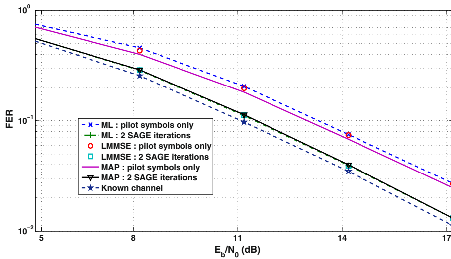
Figure 2 The FER for several estimation algorithms.
