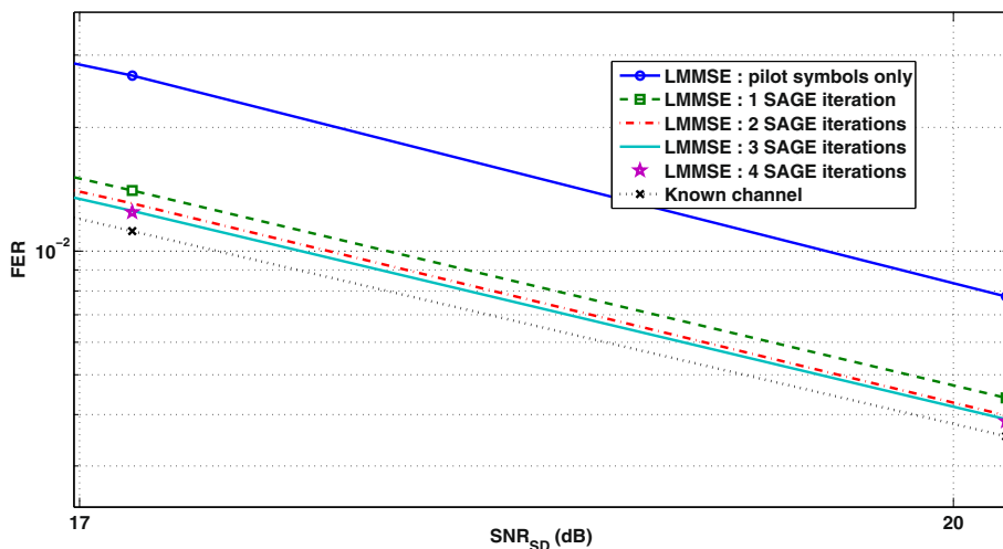
Figure 3 The FER performance of the LMMSE algorithm for several SAGE iterations.
