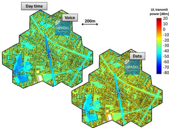
Figure 3: Tx power (dBm) calculated indoor at ground floor and outdoor during the day for voice and data traffic
