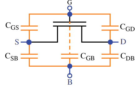
Fig. 7. Simplified schematic of the main capacitances of a MOS transistor.
