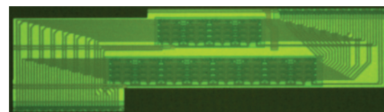
Fig. 2. Photography of the processed cascade of reversible adders (approximately 1400 \mu\text{m} \times 350 \mu\text{m} ). The two sub-blocks are visible, as well as the two multiplexer lines.
