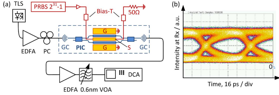
Fig. 4. Experimental setup for demonstrating the EO effect of a hybridly integrated organic crystal. Optical on-chip connections are in blue, electrical connections are drawn in red. (a) CW light from a tunable laser source (TLS) is amplified by an erbium-doped fiber amplifier (EDFA), polarization-controlled (PC), and coupled by a grating coupler (GC) to one input of a multimode interference (MMI) coupler. The MMI maps the light onto the two arms of the Mach-Zehnder interferometer modulator with phase modulators in its arms as discussed in Fig. 2. Another MMI recombines the fields. This light is coupled back to a fiber by means of a GC and guided to the receiver. The receiver consists of an EDFA, a filter and a digital communication analyzer (DCA). A pseudo-random binary sequence (PRBS) is amplified, and passed through a bias-T for adjusting the MZM to the quadrature operating point. Ground-signal-ground (GSG) electrodes excite an electrical traveling wave, which modulates the incoming light, which is evaluated in the receiver. (b) Eye diagram of the received optical signal at 12.5 Gbit/s. A quality factor Q^2 corresponding to 14 dB evaluates to a bit error ratio (BER) of 3 \times 10^{-7} .
