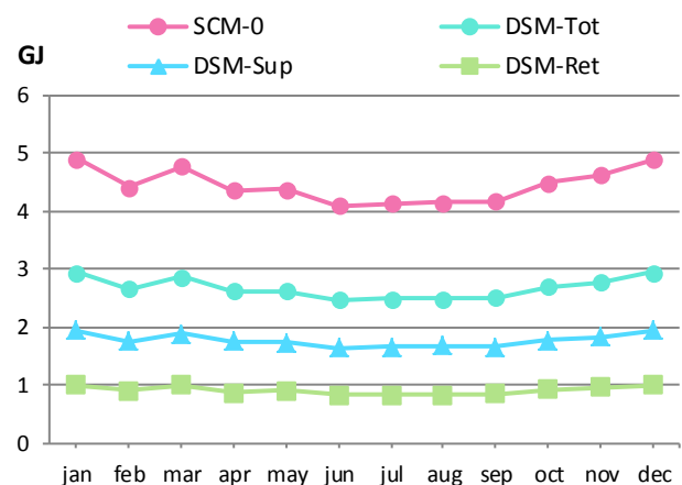
Fig. 5: Heat loss calculations: DSM and SCM-0
