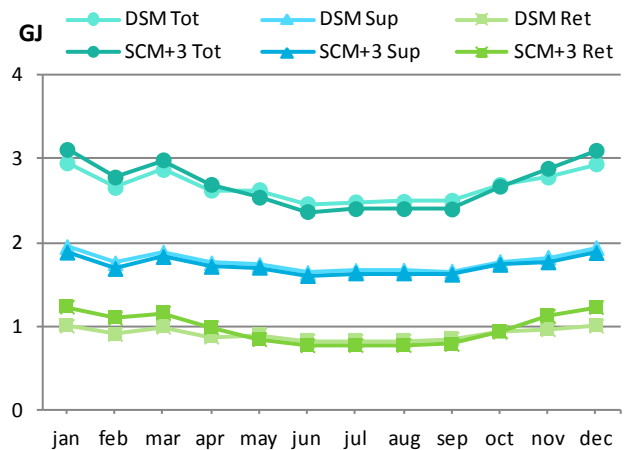
Fig. 9: Heat loss calculations: DSM and SCM+3
