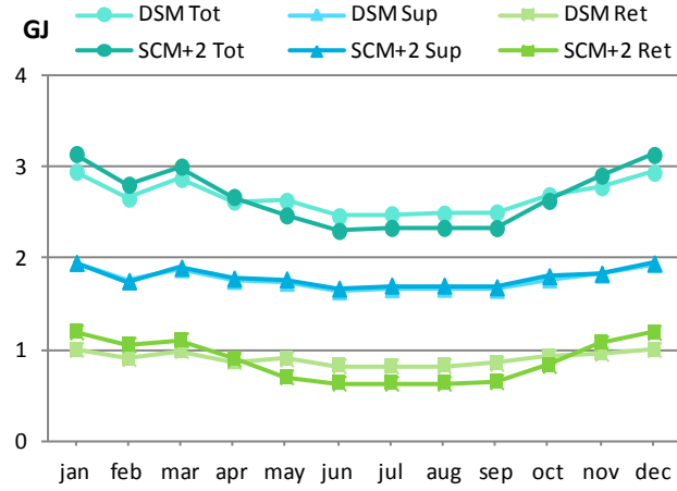
Fig. 8: Heat loss calculations: DSM and SCM+2
