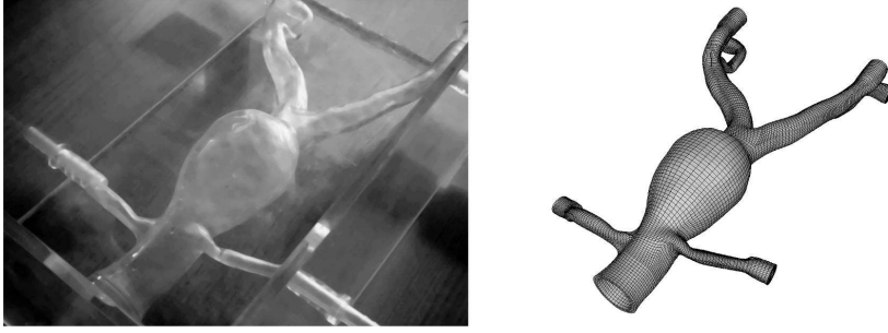
FIGURE 5.2: Silicone model (l.) and discretized FEA model (r.).
