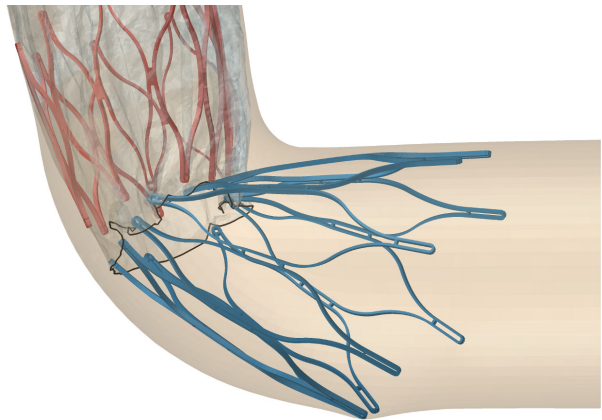
FIGURE 4.7: A finite element rendering of a deployed configuration of the device for the case of an oversize of 20%, angulation of 80.0° and translation of 35 mm (simulating a \beta angle). The device position is unstable, with a kink between the first and second stent segment, reducing the entry area of the graft (black outline).
