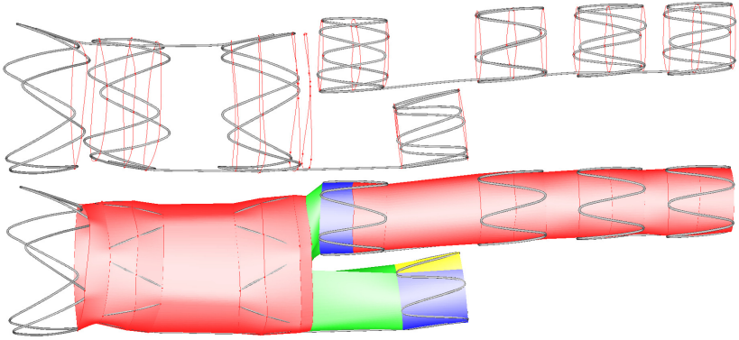
FIGURE 2.10: Modeling of the covering stent membrane. Spline curves are fit through points on the stent rings (top), and are connected to form surfaces (bottom). Visualization of the method for the Talent stent graft.
