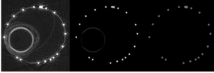
FIGURE 2.3: \mu CT slice of a scanned stent graft. Full ranged window view (left), altered window level and reduced width (middle), rainbow color lookup table, showing a good threshold for wire separation.
